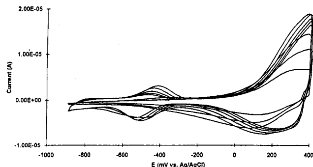
Figure 1. Cyclic voltammograms of PNMP-AQS (120 nm) in TEACl/aq. at 50 mV/s. The top CV was obtained after 30 cycles and successively after 50, 60, 70, 80, 120, 140, 150 cycles.
