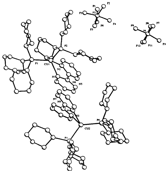
Figure 2. Relative orientation of the two independent [(\text{C}_3\text{P})_2\text{Cu}(\text{bpm})]\text{PF}_6 complexes.
