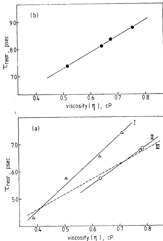
Figure 1. Viscosity dependence of \tau_{reor} for tumbling of HFB. In (a), \tau_{reor} data in neat liquid (curve III) and in neutral solvents (curves I and II) are shown. HFB mole fractions are 0.4 and 0.8 for curve I and curve II, respectively. Figure (b) is for HFB (0.4 mole fraction) in benzene (0.4 mole fraction) and neutral solvents.
