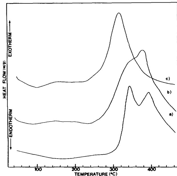
Figure 1. Differential scanning calorimograms of poly(enaryloxynitriles): a) P_6 , b) P_{16} and c) P_5 .
