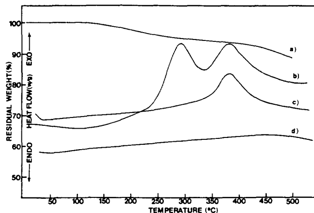
Figure 2. Differential scanning calorimogram and thermogravimogram of polymer P_{14} : a) Thermogravimogram, b) first scan, c) second scan after heating at 310\text{ }^\circ\text{C} and d) 2nd scan after heating at 390\text{ }^\circ\text{C} .
