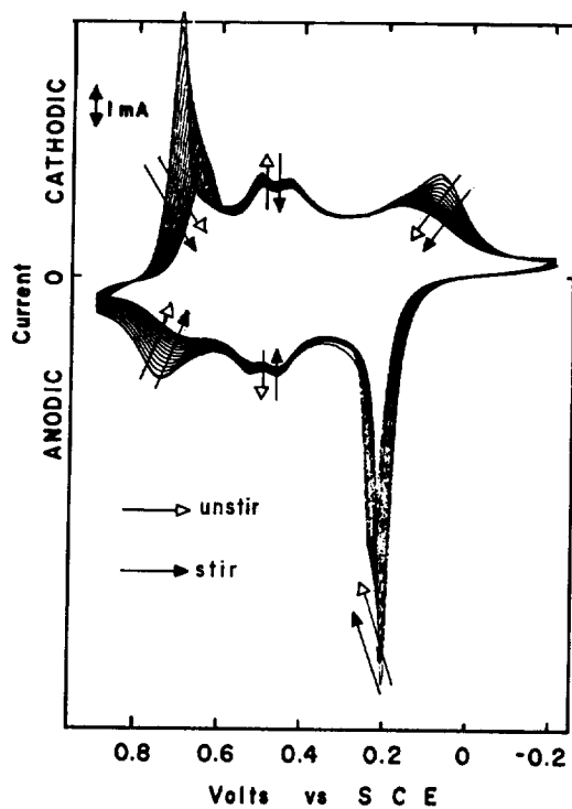
Figure 1. Cyclic voltammograms of polyaniline in 1.0M H_2SO_4 .
