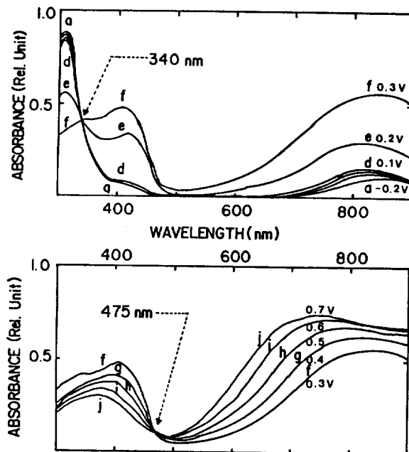
Figure 2. Visible spectra of polyaniline film coated on ITO electrode at -0.2 (a), 0.1 (b), 0.0 (c), 0.1 (d), 0.2 (e), 0.3 (f), 0.4 (g), 0.5 (h), 0.6 (i), and 0.7 \text{ V} (j).
