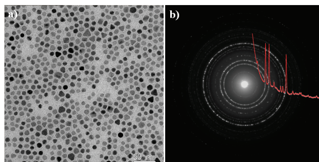
Figure 1. Bright-field image of \text{MnFe}_2\text{O}_4 nano-crystalline and the corresponding selected area electron powder diffraction. The overlay on the electron diffraction shows the average intensity profile that was used to determine the structure.
