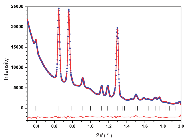
Figure 3. Rietveld analysis of the electron powder diffraction from \text{MnFe}_2\text{O}_4 nano-crystalline. The positions of the Bragg reflections are indicated by vertical bars (|). The difference between the experimental (dots) and the calculated (solid line) intensities from the refined model is shown by the plot in the lower part of the diagram.
