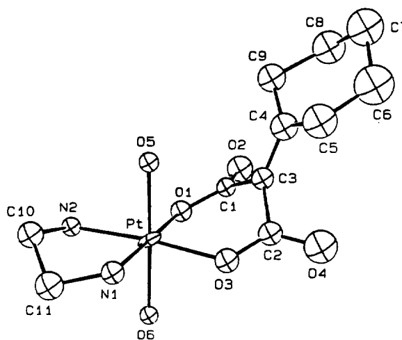
Figure 1. ORTEP drawing of the complex 5 .
