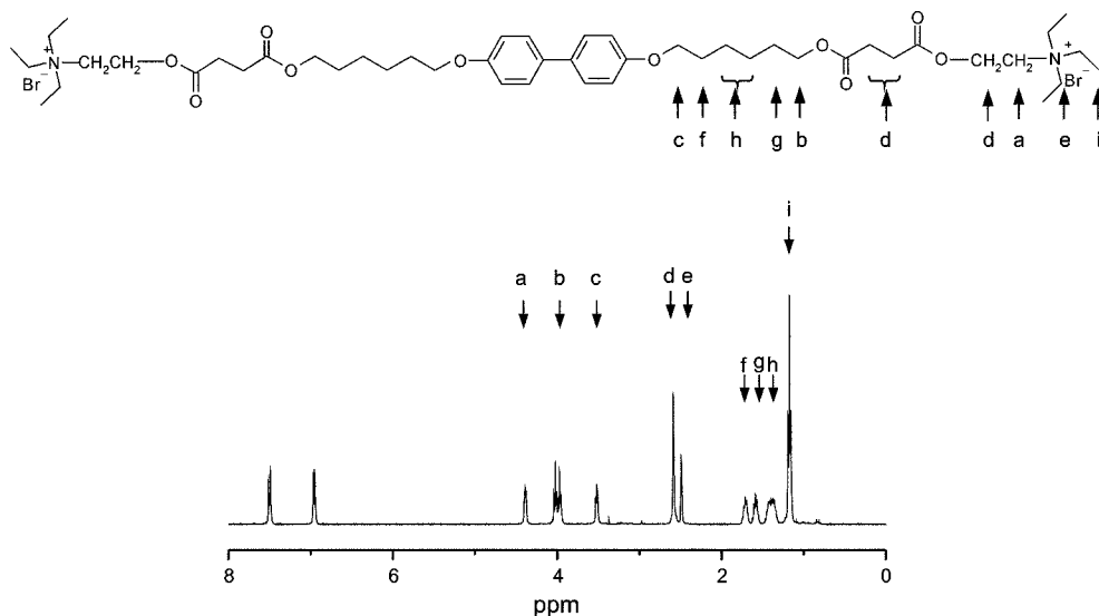
Figure 3. 1 H-NMR (DMSO- d 6 ) spectrum of BPAS.
