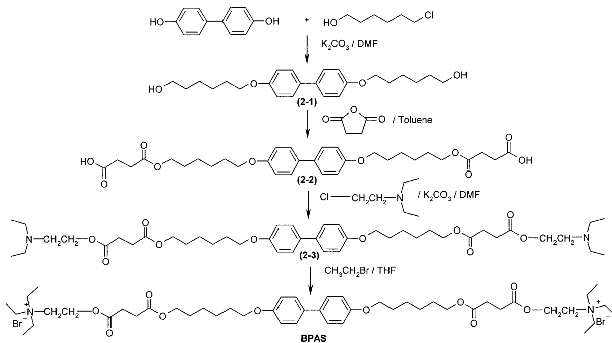
Scheme 2. Synthetic route to BPAS.
