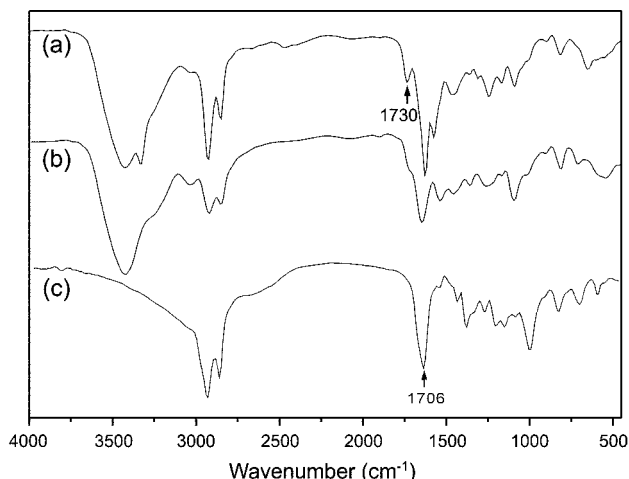
Figure 7. FT-IR spectra of large vesicles after (a) polymerization, (b) skeletonization, and (c) hydrolysis.
