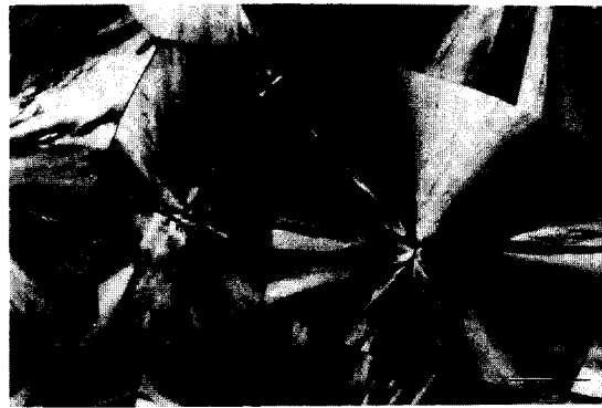
Figure 6. A polarizing optical micrograph (43 \mu\text{m} scale bar) of PTMS spherulites grown at 100 °C.
