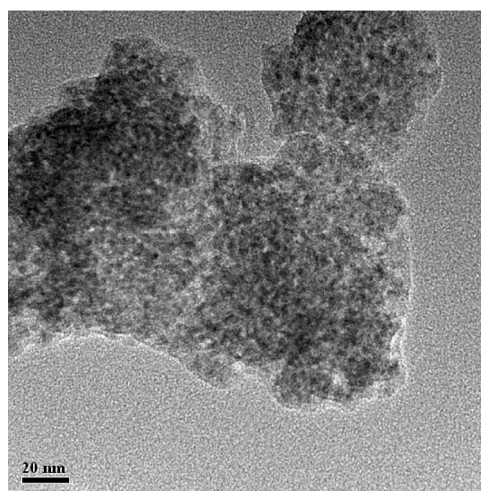
Specimen : Operator : Voltage : 300 kV Microscope Name : JEM-3011 Name : US1000 1 Total Magnification : X920000 Indicated Magnification : X100000 Image Name : Frame Resolution : 2048 x 2048 pixels Acquisition Date : 2006-07-21 Acquisition Time : 2006-07-21 1:15:54 Collection Number : Exposure Time : 0.5 s Image Notes :
