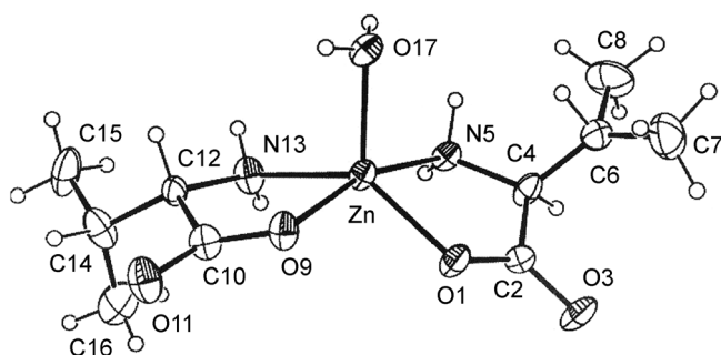
Figure 1. The ORTEP view of [\text{Zn}(\text{val})_2(\text{H}_2\text{O})] including the atom numbering scheme. (30% ellipsoid probability); Selected bond lengths (Å) and angles ( ^\circ ): Zn-O(1) 2.017(2), Zn-O(9) 2.062(2), Zn-O(17) 2.034(3), Zn-N(5) 2.107(3), Zn-N(13) 2.077(4); O(1)-Zn-N(5) 80.83(10), O(9)-Zn-N(13) 80.67(11), O(1)-Zn-O(9) 86.66(10), N(5)-Zn-N(13) 102.50(13), O(1)-Zn-O(17) 120.51(12), O(9)-Zn-O(17) 99.57(12), O(17)-Zn-N(5) 94.99(14), O(17)-Zn-N(13) 100.64(16), O(1)-Zn-N(13) 138.44(16), O(9)-Zn-N(5) 164.28(12).
