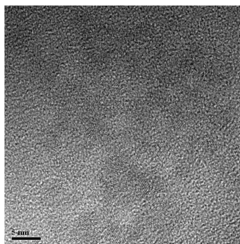
Specimen : Operator : Voltage : 300 kV Microscope Name : JEM-3011 Name : US1000 1 Total Magnification : X4590000 Indicated Magnification : X500000 Image Name : Frame Resolution : 2048 x 2048 pixels Acquisition Date : 2006-07-21 Acquisition Time : 2006-07-21 1:18:47 Collection Number : Exposure Time : 0.5 s Image Notes :
