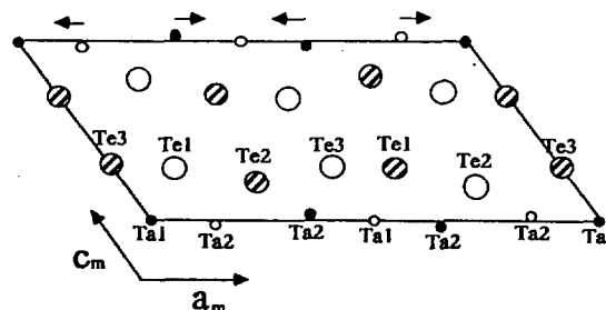
Figure 4. Projection of MTe_2 ( M = Ta, Nb, V ) structure onto (010) face. Large open circles are tellurium atoms at y = 1/2 , hatched circles are tellurium atoms at y = 0 . Small open circles are metal atoms at y = 1/2 and closed circles are metal atoms at y = 0 . The directions of displacements of the M(2) atoms from their positions in the CdI_2 -type structure are indicated by arrows.
