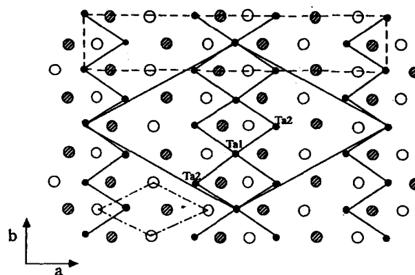
Figure 3. Projection of a single MTe_2 ( M = Ta, Nb, V ) layer on (001) face in a direction perpendicular to (001). Closed circles are metal atoms. Open circles are tellurium atoms above, and the hatched circles are tellurium atoms below the metal atom sheet, respectively. The shortened metal-metal distances are emphasized by solid lines. The cell of the monoclinic superstructure is indicated by dotted lines and hexagonal superstructure with a = 3a_h (where a_h is unit cell parameter of CdI_2 -type structure) is indicated by solid lines. Pseudo-hexagonal subcell (ideal CdI_2 -type structure) is indicated by broken lines.
