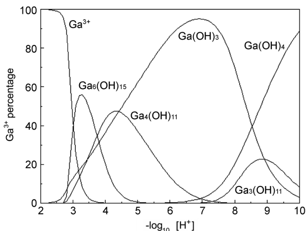
Figure 4. Simulated distribution of the Ga(III) into its free and hydroxylated species as a function of pH, with Ga(III) = 2 mmol·dm -3 .
