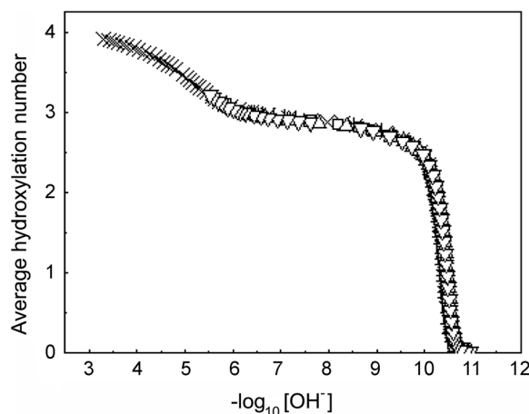
Figure 2. Simulated hydroxylation curves relative to Ga(III) as obtained by means of SIMDIS program using results in Table 2 (i); key to symbols as in Table 1.
