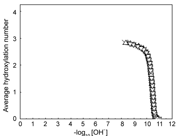
Figure 3. Simulated hydroxylation curves relative to Ga(III) as obtained by means of SIMDIS program using results in Table 2 and data pairs limited to pH ca. 5.0; key to symbols as in Table 1.
