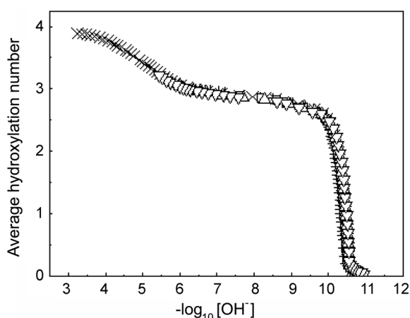
Figure 1. Experimental hydroxylation curves relative to Ga(III); key to symbols as in Table 1.
