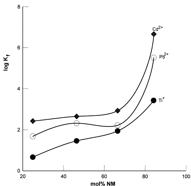
Figure 4. Variation of \log K_f of DB18C6 complexes with \text{Pb}^{2+} , \text{Cd}^{2+} and \text{Tl}^+ ions in NM/DMSO binary systems.
