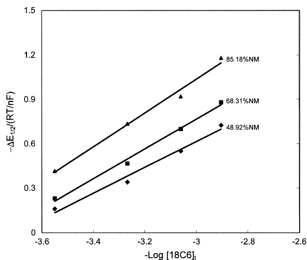
Figure 1. Linear plots of \Delta E_{1/2}/(RT/nF) versus \log [18C6]_t for the 18C6-TI + complex in DMF-NM binary mixtures.
