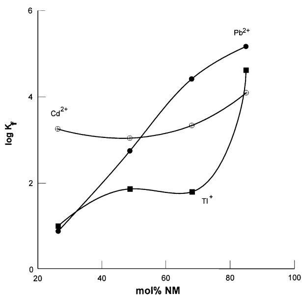
Figure 5. Variation of \log K_f of DB18C6 complexes with \text{Pb}^{2+} , \text{Cd}^{2+} and \text{Tl}^+ ions in NM/DMF binary systems.
