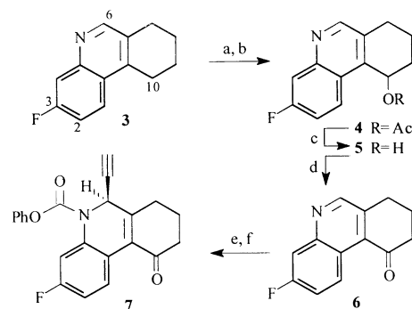
Scheme 1. C6 and C10 functionalization of tricyclic compound. Reagents and conditions: (a) 2.0 equiv of H 2 O 2 , AcOH, 70 °C, 8h, 78%; (b) Ac 2 O, 25 °C, 2 h, 90%; (c) K 2 CO 3 (cat.), MeOH, 25 °C, 5 h, 78%; (d) 1.5 equiv of PCC, CH 2 Cl 2 , 0 °C, 3h, 87%; (e) 1.2 equiv of t BuMe 2 SiOSO 2 CF 3 , 1.5 equiv of Et 3 N, CH 2 Cl 2 , 25 °C, 3h, 94%; (f) 1.2 equiv of ethynylmagnesium bromide, 1.1 equiv of PhOCOCl, THF, -78 °C to 25 °C, 40 min and then, 10% HCl, 25 °C, 12h, 100%.
