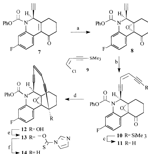
Scheme 2. Synthesis of a new dynemicin A model 14 . Reagents and conditions: (a) 1.2 equiv of m CPBA, aq. NaHCO 3 /CH 2 Cl 2 , 25 °C, 30 min, 64%; (b) 1.6 equiv of 9 , 0.06 equiv of Pd(PPh 3 ) 4 , 0.24 equiv of CuI, 2.0 equiv of n BuNH 2 , benzene, 25 °C, 1 h, 80%; (c) 4.0 equiv of AgNO 3 , 7.0 equiv of KCN, THF/EtOH/H 2 O, 25 °C, 25 min, 86%; (d) 1.0 equiv of LDA, toluene, -78 °C, 10 min, 75%; (e) 3.0 equiv of thiocarbonyldiimidazole, 0.6 equiv of DMAP, CH 2 Cl 2 , 25 °C, 24 h, 56%; (f) 2.0 equiv of t Bu 3 SnH, AIBN (cat.), toluene, 80 °C, 1h, 83%.
