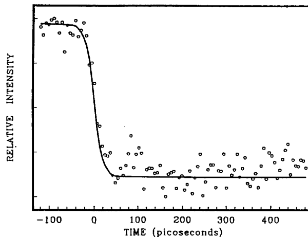
Figure 2. Dynamics for the intensity change of the negative-going peak at 533 \text{ cm}^{-1} . Positive times correspond to pump followed by delayed probe. Relative energies are approximately 15 \mu\text{J} for the pump and 3 \mu\text{J} for the probe. Step size of the optical delay is 5 ps. The solid line through the data represents a 5 ps decay time.
