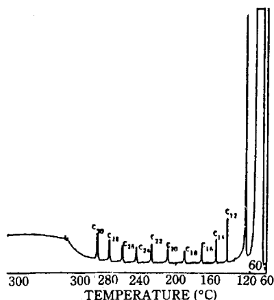
Figure 3. Gas chromatogram of n-hydrocarbons on a Chromosorb W packed column (0.9 m × 2 mm ID) 5% SE-54 cross-linked with 1% dicumylperoxide. 1 \mu l cold on-column injected; column temperature, 60°C until hexane peak, then raised to 120°C and programmed to 300°C at 10°C/min; 30 ml/min of helium.
