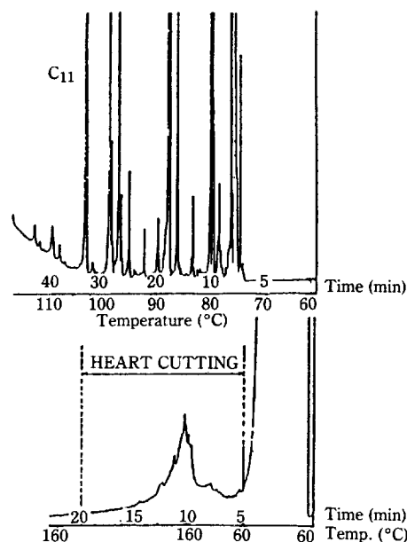
Figure 5. Gas chromatograms of hexane impurities preconcentrated (Bottom) on a cross-linked packed column (0.9 m × 2 mm ID) then analyzed (Top) on a Witconal capillary column (100 m × 0.5 mm ID). Chromatographic conditions in text.
