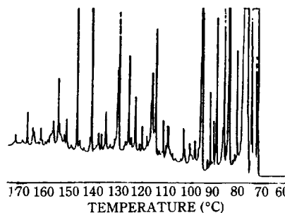
Figure 6. Gas chromatogram of serum volatile metabolites on a witconal capillary column (100 m × 0.5 mm ID) after their trace enrichment on the cross-linked Chromosorb W. Same conditions as in Figure 5.
