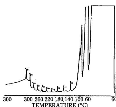
Figure 4. Gas chromatogram of n-hydrocarbons on a Chromosorb W packed column (1.8 m × 2 mm ID) 5% SE-54 cross-linked with 1% dicumylperoxide. 100 \mu l of hexane spiked with n-hydrocarbons at 0.2 ppm, cold on-column injected; 30 ml/min of helium; column temperature, 60°C until hexane peak, then programmed to 300°C at 10°C/min.
