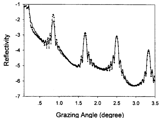
Figure 2. Reflectivity vs. \theta of cadmium arachidate LB film: \cdots , measurement; - , calculation.
