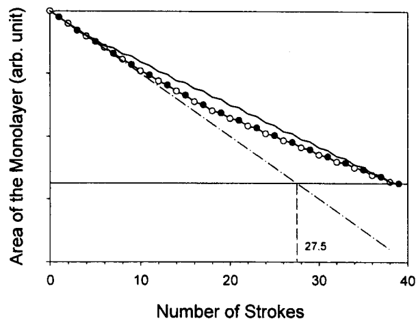
Figure 1. Measured consumption of the floating monolayer of cadmium arachidate after every stroke: \circ \rightarrow \bullet , upstroke; \bullet \rightarrow \circ , downstroke, -\cdot-\cdot- , Y-type deposition, - , simulation curve of monolayer consumption.
