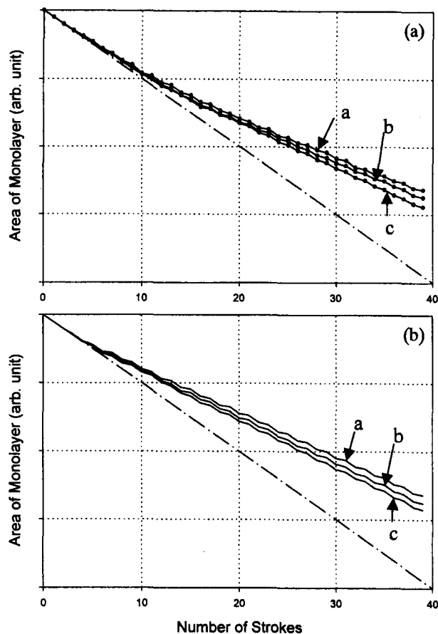
Figure 8. Consumption of floating monolayer after every stroke: (a) Measurement; (b) Simulation; curve a, cadmium stearate; curve b, cadmium arachidate; curve c, cadmium beheniate; \text{---} , Y-type deposition.
