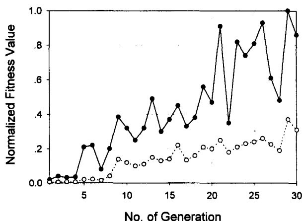
Figure 6. Fitness value of individual generation in simulation: \cdots\circ\cdots average fitness; \bullet\text{---}\bullet maximum fitness.
