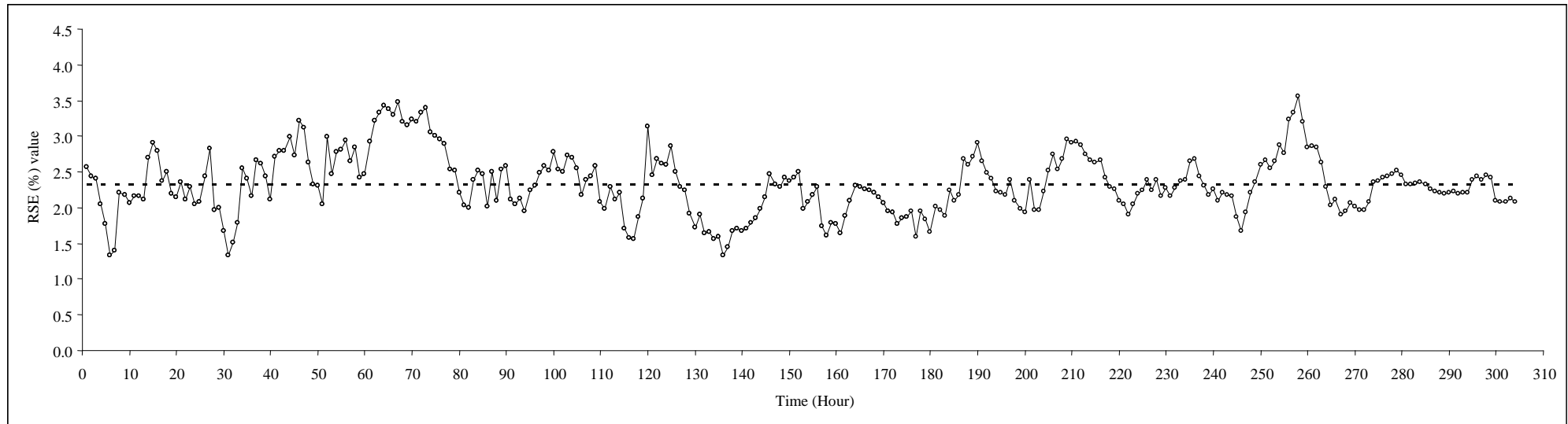
Figure 4. The variation in hourly RSE (%) values in the simultaneous measurement of CO 2 made by 6 sensor units (Dotted line shows the overall mean RSE value for the entire study).
