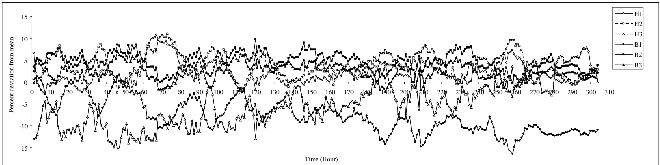
Figure 5. The temporal variation of percent deviation (PD) values derived using hourly mean value of CO 2 data measured concurrently by 6 sensor units.
