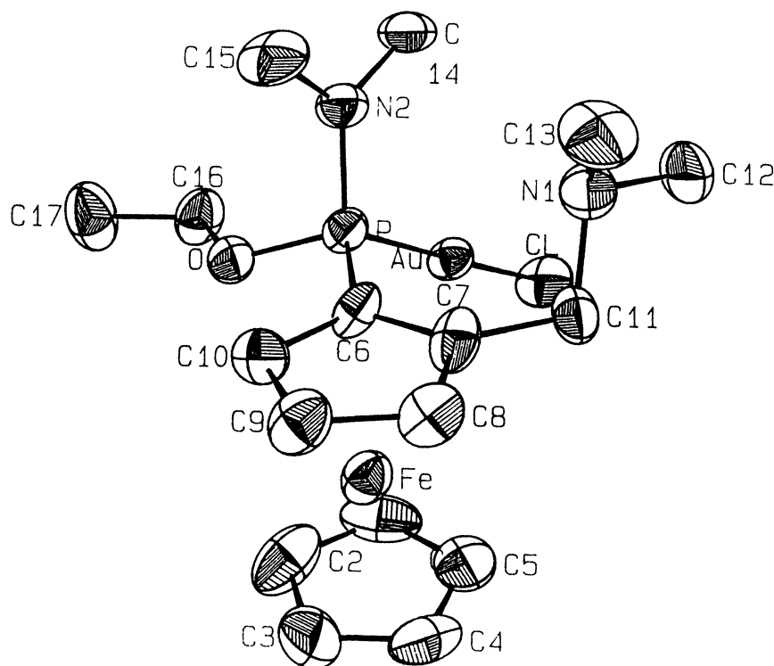
Figure 2. ORTEPdrawing of [Fc(CH 2 NMe 2 )(P(NMe 2 )(OCH 2 CH 3 )(AuCl)] (7)
