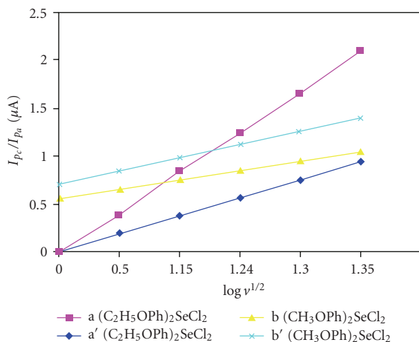
FIGURE 5: The dependence of I_{pc} and I_{pc}/I_{pa} in CV, conditions: 0.1 M TBABF 4 in CH 3 CN.
