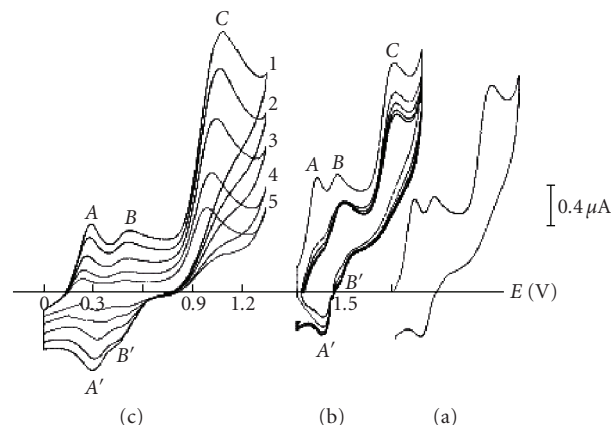
FIGURE 1: (a) Cyclic voltammogram of 0.004 M (C 2 H 5 OPh) 2 SeCl 2 ; (b) cyclic voltammogram of 0.0035 M (CH 3 OPh) 2 SeCl 2 ; (c) rate of potential scans: (1) 50 mV/s, (2) 40 mV/s, (3) 30 mV/s, (4) 20 mV/s, and (5) 10 mV/s, conditions: 0.1 M TBABF 4 in CH 3 CN.
