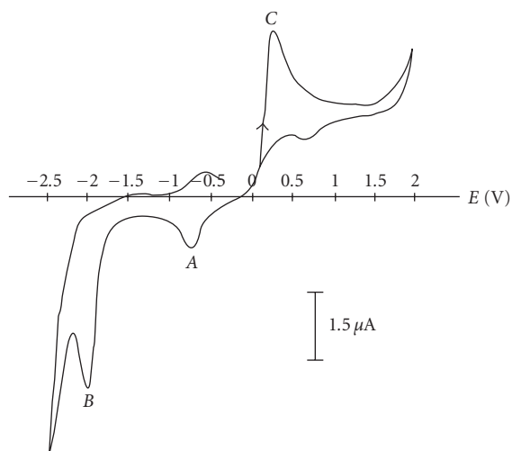
FIGURE 8: Cyclic voltammogram of 0.004 M (\text{C}_2\text{H}_5\text{OPh})_2\text{Se}_2 , conditions: 0.1 M TBAFB in \text{CH}_3\text{CN} . Potential scan rate: 100 mV/s.
