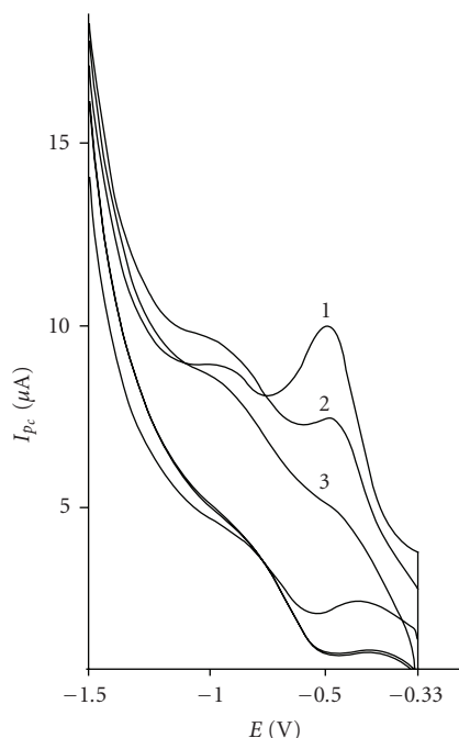
FIGURE 2: The cyclic voltammograms of AN containing 2 mM \text{Ar}_2\text{SeCl}_2 at stationary platinum electrode ( 2.5 \text{ cm}^2 ): (1) at the beginning, (2) during, (3) and at the end of electrolysis. Supporting electrolyte: 0.1 M TBAFB, scan rate: 100 mV/s.
