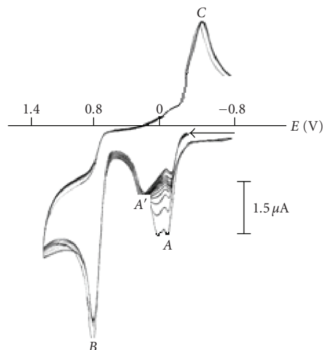
FIGURE 6: Multisweep-cyclic voltammograms of 0.0025 M (\text{C}_2\text{H}_5\text{OPh})_2\text{Se}_2 , conditions: 0.1 M TBABF 4 in CH 3 CN. Scan rate 100 mV/s.
