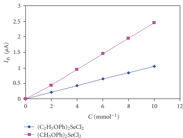
FIGURE 4: The dependence of the peak currents of the concentrations, conditions: 0.1 M TBABF 4 in CH 3 CN.
