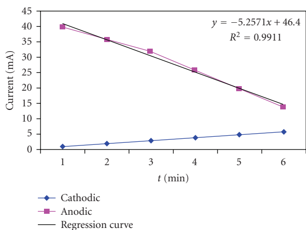
FIGURE 3: Changes with respect to time in the oxidation and reduction peaks of bis(pethoxyphenyl) selenium dichloride ( \text{Ar}_2\text{SeCl}_2 ) electrolyzed at constant potential -1.1 \text{ V} , cathodic and anodic current curves.
