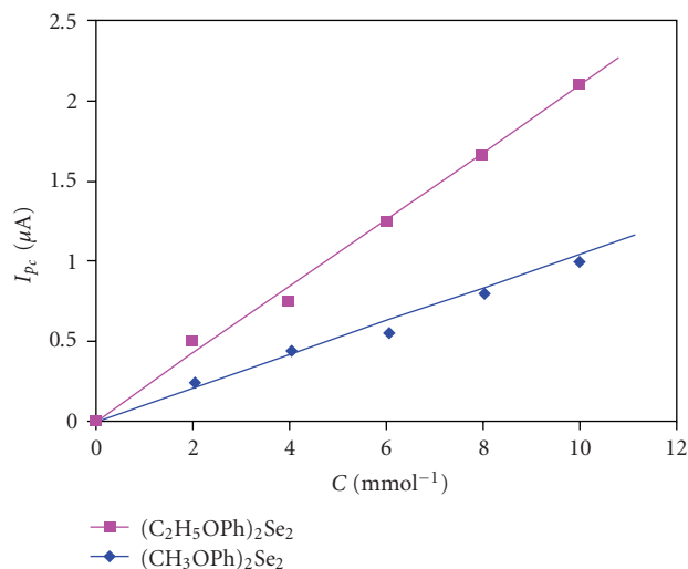
FIGURE 9: The dependence of the limiting currents of the waves on the concentrations.
