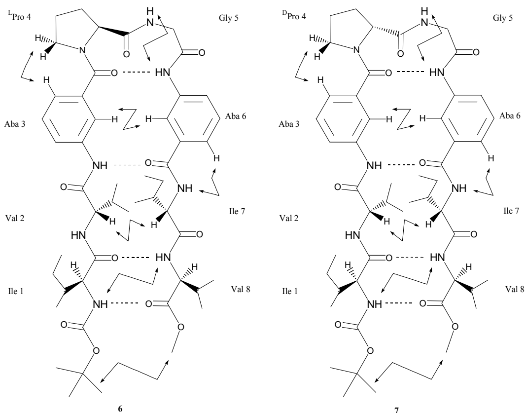
Figure 3. Schematic representation of NOEs and H-bonds for 6 and 7 .
