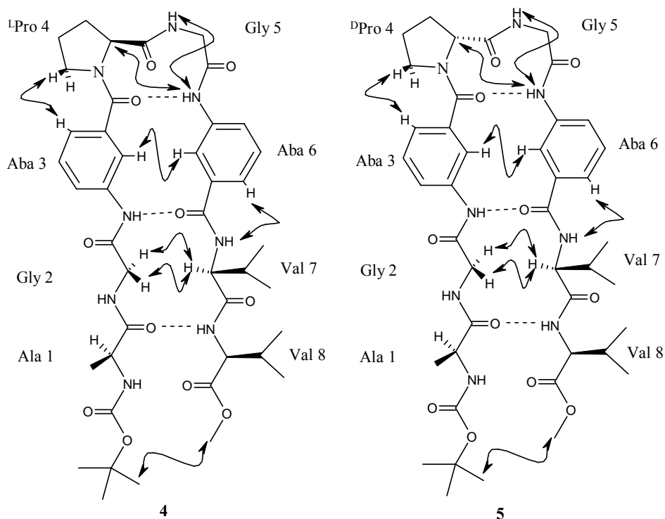
Figure 2. Schematic representation of NOEs and H-bonds for 4 and 5 .
