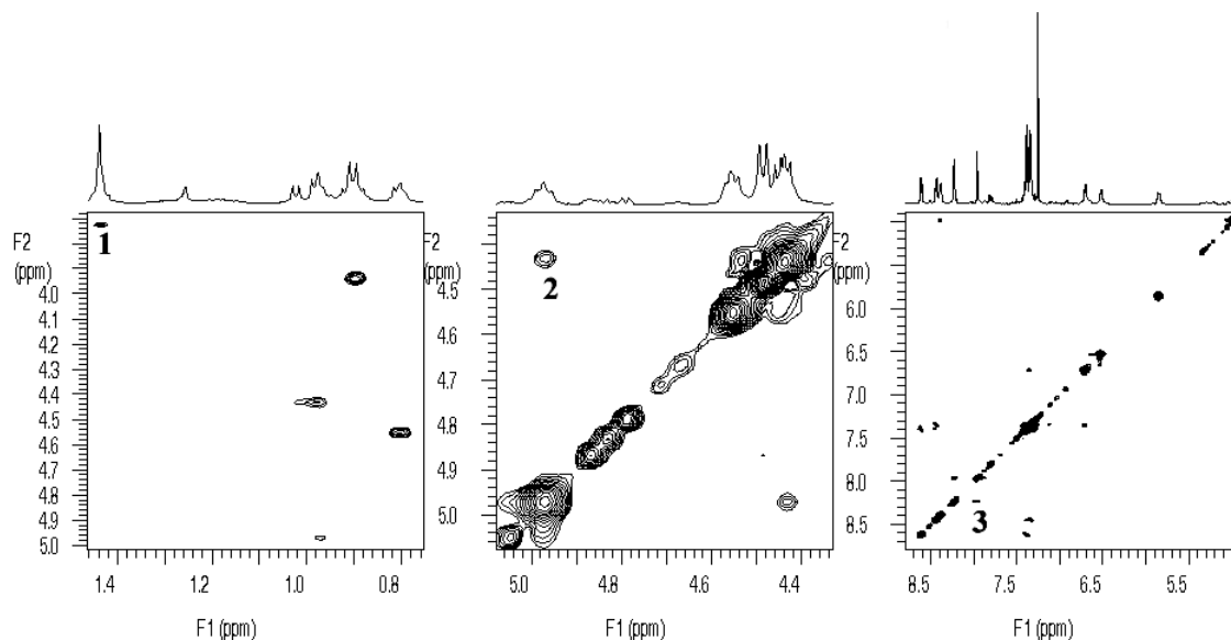
Figure 5. Expanded ROESY spectrum of peptide 8 . The NOE cross peaks are: (1) Boc / OCH 3 , (2) Val2αH / Ile7αH and (3) Aba3H2 / Aba6H2.
