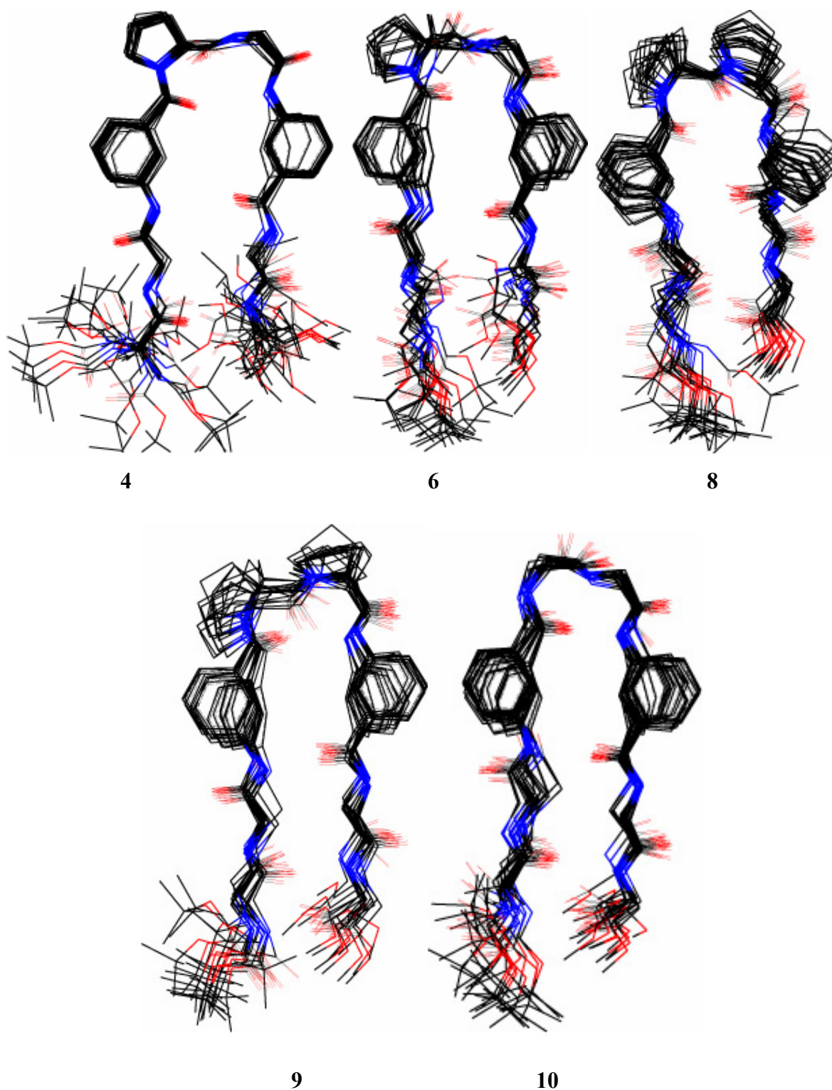
Figure 7.20 Overlapped structures obtained from molecular dynamics simulation studies for 4, 6, 8, 9 and 10. For clarity in visualization the side chain groups are not shown in the figure except for proline.
