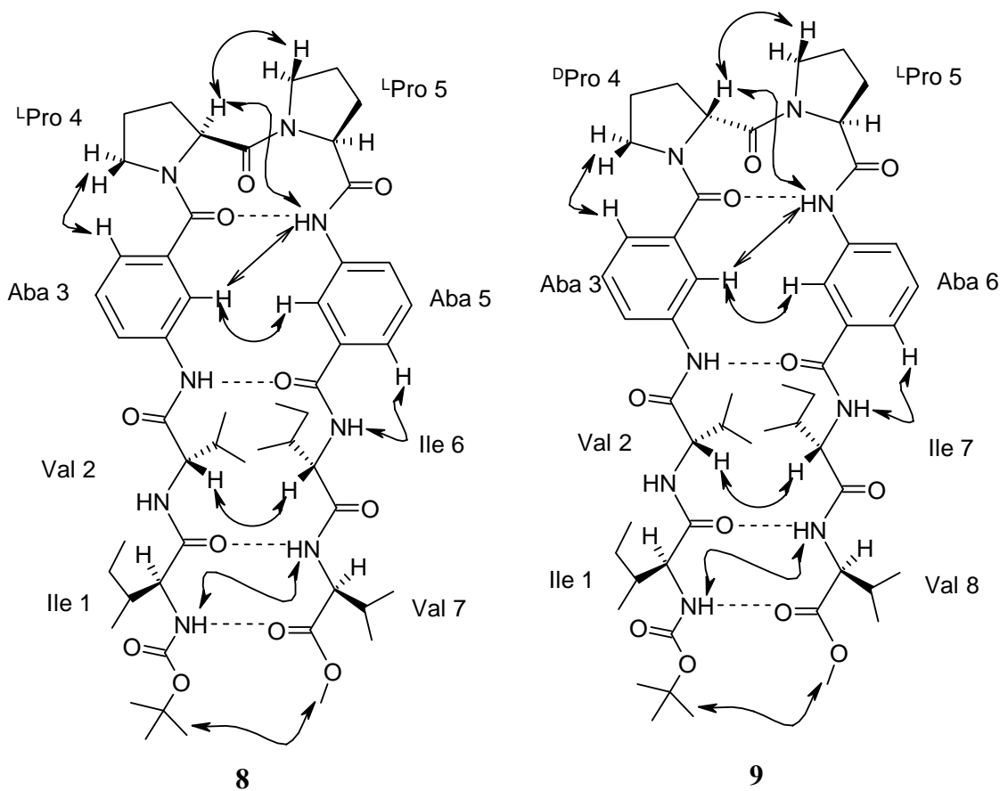
Figure 4. Schematic representation of NOEs and H-bonds for 8 and 9 .
