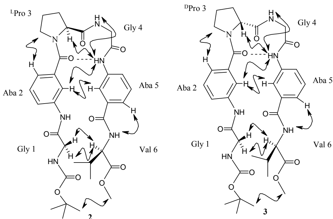
Figure 1. Schematic representation of NOEs and H-bonds for 2 and 3 .
