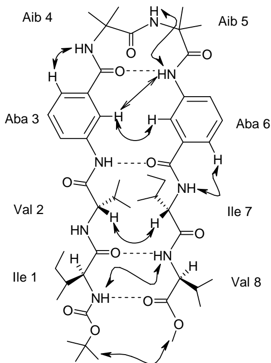
Figure 6. Schematic representation of NOEs and H-bonding for 10 .
