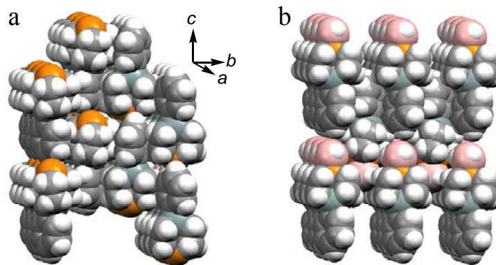
Figure 3. Crystal packing of Ph-SMAP ( 1a , a) and Ph-SMAP-BH 3 ( 12 , b).
