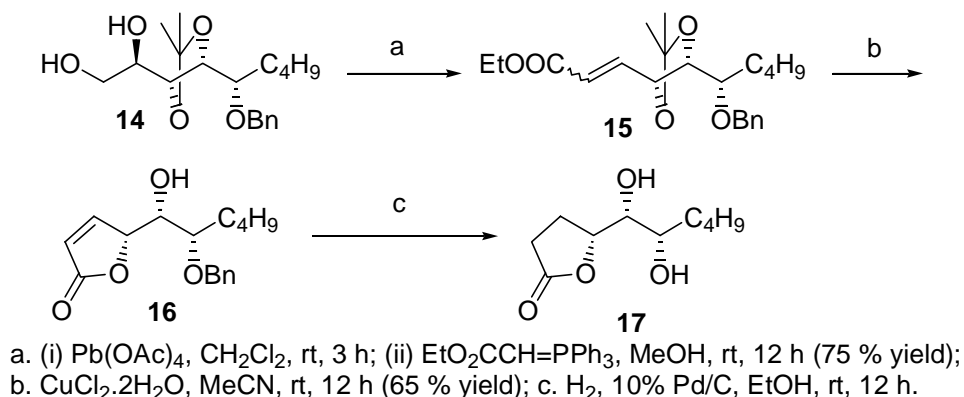
Scheme 4. Synthesis of 17 .
