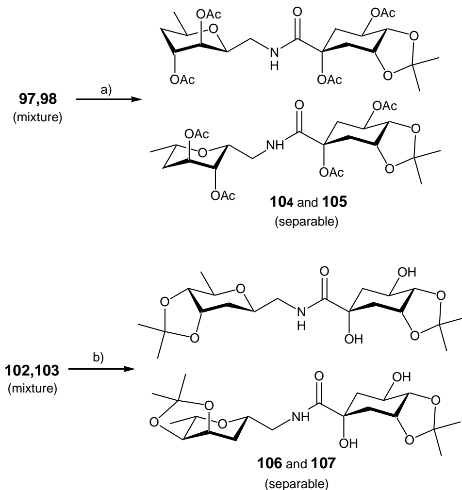
Scheme 16. Separation of diastereomeric mixtures of quinamides as isopropylidene-tetra-O-acetyl or diisopropylidene derivatives: (a) \text{Ac}_2\text{O} , DMAP, Py; (b) 2-methoxypropene, p -TsOH, DMF. 49,128
