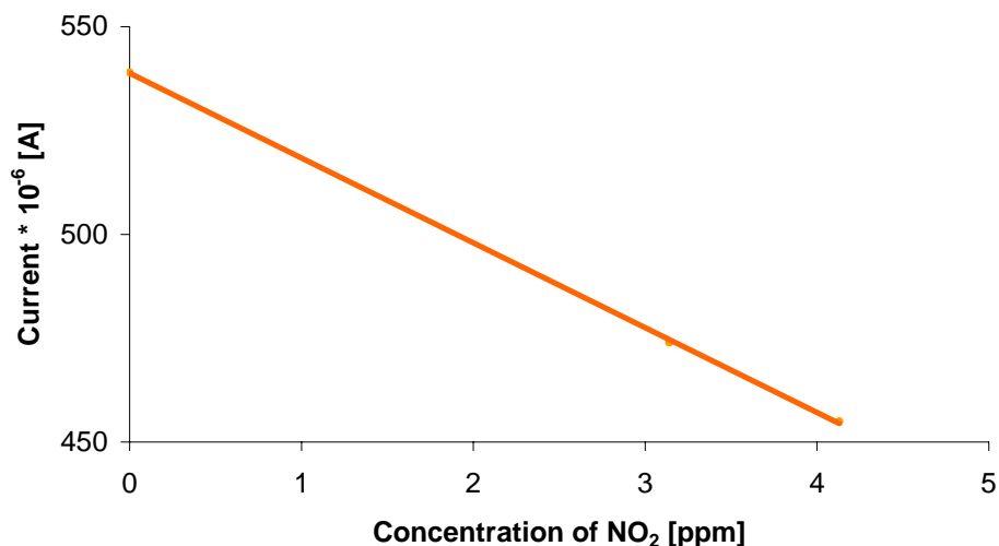
Figure 4. Conductivity response of 5 layer LB film on increasing \text{NO}_2 concentration in atmosphere surrounded the sample. U = 15 mV.
