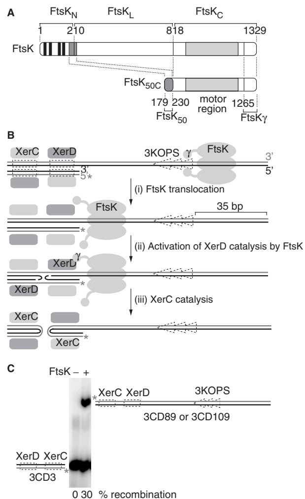
Figure 1. Asymmetric Xer recombination assay. (A) Schematic of E. coli FtsK. The positions of the amino acid residues delimiting the different domains of the protein are indicated. Black bars depict the transmembrane domains. (B) Recombination between a long substrate containing a triple KOPS motif (3KOPS) oriented towards dif and a short radiolabelled dif probe. Top and bottom strands are depicted as grey and black lines, respectively. The 5' and 3' indicate the polarity of the strands. The radioactive label on the short substrate is indicated by a star. FtsK loads on the KOPS, translocates (i) and activates catalysis by the XerD recombinases (ii), leading to the formation of Holiday junction. The XerD recombinases cleave the bottom strands. The XerC recombinases then cleave the top strands (iii). The resulting products are a short unlabelled probe and a long radiolabelled fragment. (C) Recombination reaction between 3CD3 and 3CD89.
