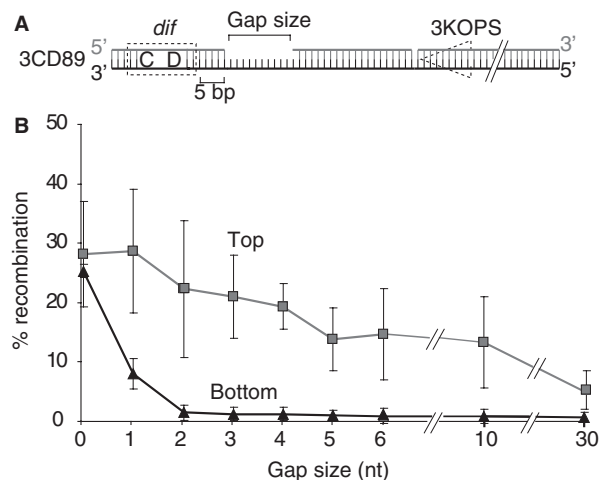
Figure 4. A 2 nt gap on the bottom strand of DNA stops recombination activation. Efficiency of recombination (B) using substrates with variable gap size at 5 nt from dif (A).
