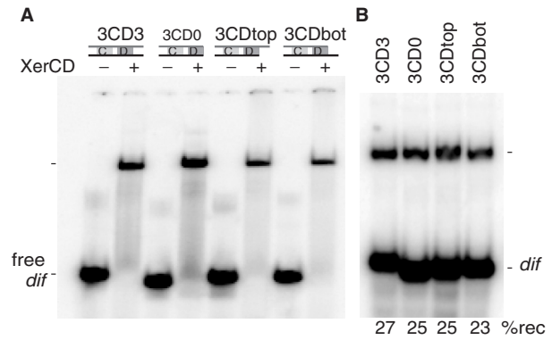
Figure 6. The duplex DNA adjacent to dif is not required for XerCD binding and activity. (A) Gel mobility shift assay showing equivalent binding of XerCD recombinases on short dif substrates: 3CD3 carries 3 bp on the XerD side of dif , 3CDtop and 3CDbot, respectively, carry 3 nt of single-stranded DNA on the top or bottom strands of DNA on the XerD side of dif , 3CD0 entirely lacks DNA on the XerD side of dif . (B) PAGE showing equivalent recombination efficiency between 3CD89 and 3CD3, 3CD0, 3CDtop or 3CDbot.
