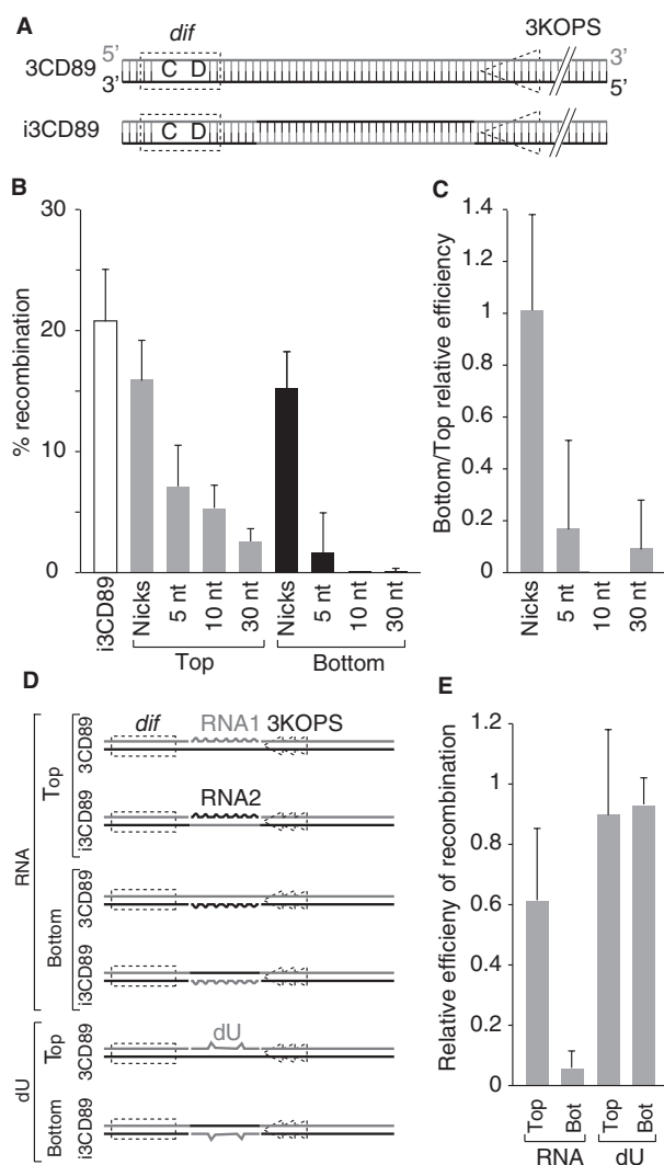
Figure 3. Top- and bottom-strands asymmetry is not linked to base composition. (A) Scheme of i3CD89 recombination substrates, which present a 30-bp inverted region between dif and the 3KOPS motif compared to 3CD89 substrates. (B) Efficiency of recombination for the different i3CD89 substrates (mean and standard deviations of four independent experiments). (C) Relative efficiency of recombination of i3CD89 substrates with bottom-strand gaps versus substrates with top-strand gaps (mean and standard deviations of four independent experiments). (D) Scheme of 3CD89 and i3CD89 recombination substrates with 30-nt gaps on top or bottom strand filled with RNA or DNA containing deoxyuridines (dU). (E) Relative efficiency of recombination of RNA and dU substrates (the number of independent experiments are indicated upon each data column). No differences were observed between 3CD89 and i3CD89 RNA substrates and results were pooled.
