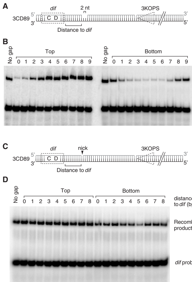
Figure 5. Scanning for important nucleotides in the immediate vicinity of dif . 3CD89 recombination substrates presenting 2 nt gaps (A–C) or nicks (D–F) at variable position from dif . Schemes of the substrates (A, C); gels displaying typical recombination results (B, D); mean efficiency of recombination from three independent experiments (E, F). The largest error bars in Figure 5F correspond to the substrates with nicks on the bottom strand.
