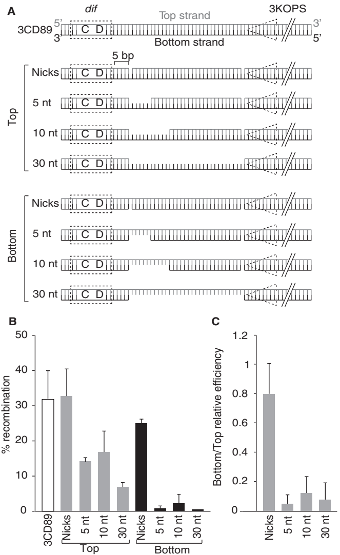
Figure 2. Top- and bottom-strand gaps affect recombination efficiency. (A) Scheme of 3CD89 recombination substrates with nicks or gaps of different length on the top or bottom strand. No phosphate residues are left at the position of nicks. (B) Efficiency of recombination for the different 3CD89 substrates (mean and standard deviations of four independent experiments). (C) Relative efficiency of recombination of substrates with bottom-strand gaps versus substrates with top-strand gaps (mean and standard deviations of four independent experiments).
