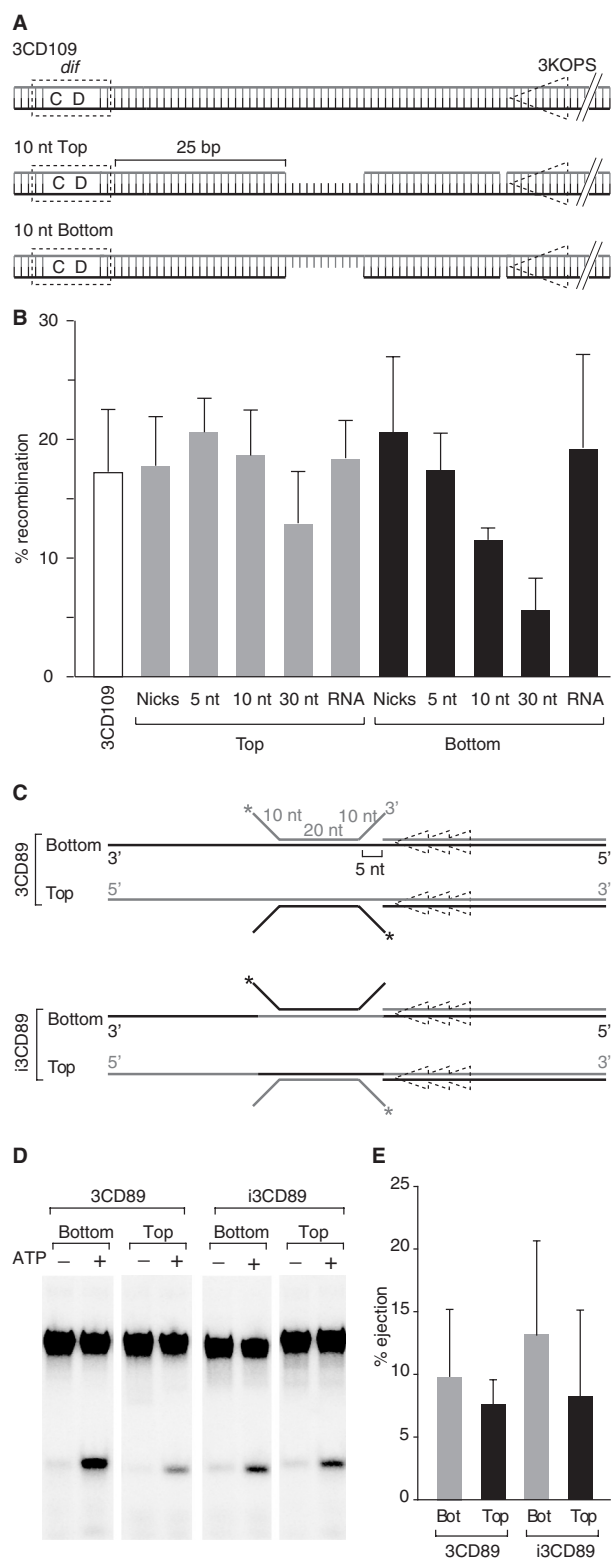
Figure 7. The effect of gaps is local. (A) Scheme of 3CD109 recombination substrates, which contain 20 more base pairs between dif and the 3KOPS motif than 3CD89 substrates. (B) Efficiency of recombination on 3CD109 substrates with gaps at 25 bp from dif (mean and standard deviations of three independent experiments). (C) Scheme of the oligonucleotide displacement substrates based on 3CD89. The loading site of FtsK (including the 3KOPS and the 35 bp tail) is double-stranded. Radiolabelled oligonucleotides are annealed to 20 bases of 3CD89 at
