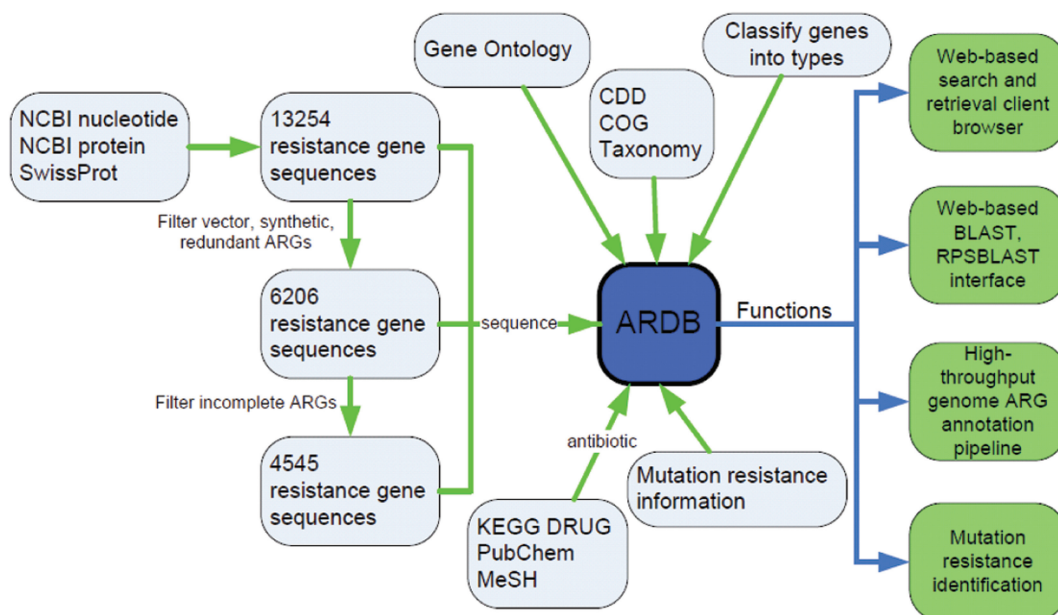
Figure 1. ARDB curation data flow.
