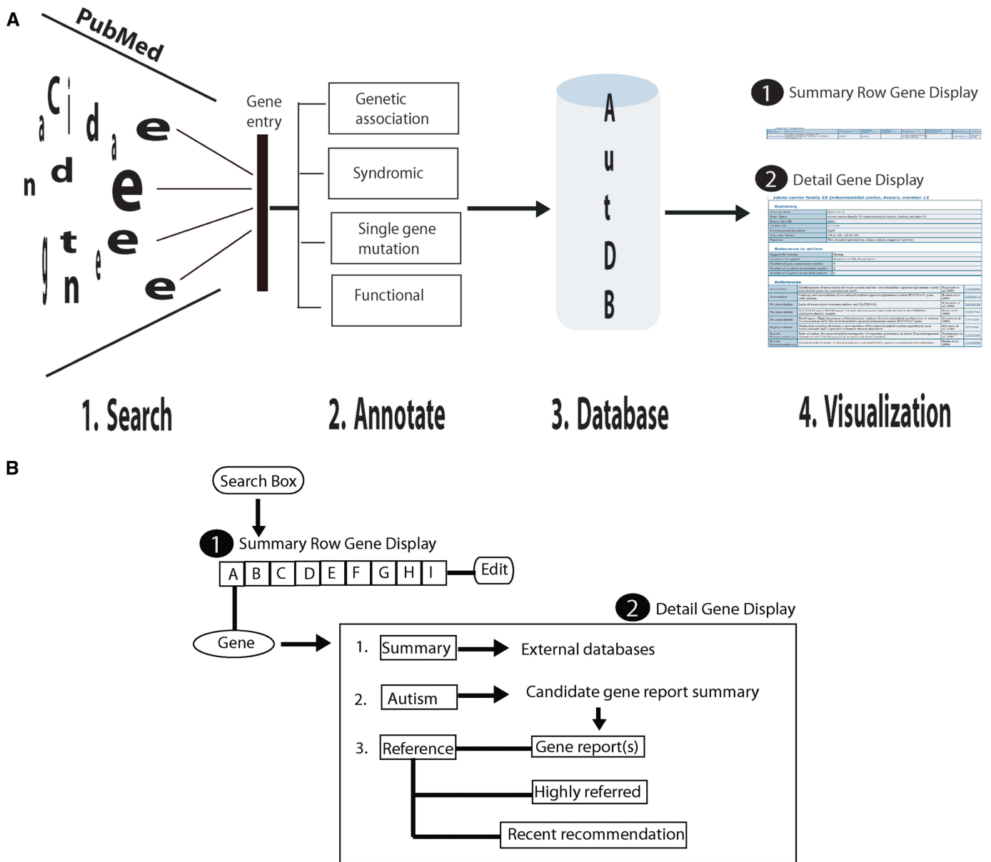
Figure 1. (A) An integrated model for collection, annotation, storage and visualization of candidate genes for ASD. (1) Candidate genes for ASD are compiled and maintained from an exhaustive search of scientific literature in the PubMed database maintained at NCBI (2) ASD candidates are classified into four categories. (3) Entries are organized in the database for search and retrieval. (4) User-friendly display of candidate genes at two levels for display and easy access with links to various external databases. (B) Search and display of candidate genes in AutDB. A search box is used to retrieve ASD candidate genes catalogued in AutDB using various gene attributes. The search results are displayed at two levels. At level 1, the gene entry is displayed in the summary row format showing: (A) gene symbol, (B) gene name, (C) chromosomal location, (D) Genetic category, (E) GAD and (F) OMIM links where available, (G) Number of autism-specific studies, (H) primary PubMed reference and (I) detail/edit button. A level 2, the entry is further displayed at a detail level in three-tier format showing: (1) gene summary with links to external databases such as Entrez Gene and UniProt, (2) relevance for autism displaying candidate gene report summary and (3) references arranged under three sub-headings: references for the candidate gene reports, highly referred and recent studies of the candidate genes.
