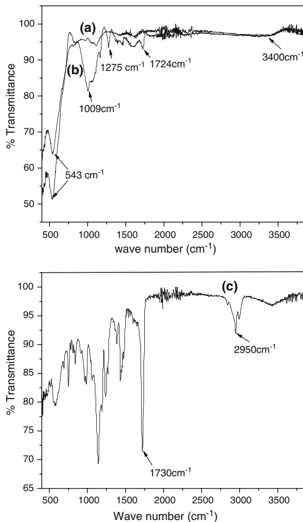
Fig. 4 RIFT-IR spectrum of (a) magnetite nanoparticle, (b) ATRP initiator-anchored magnetite nanoparticle and (c) poly(methyl methacrylate)-grafted magnetite nanoparticle
