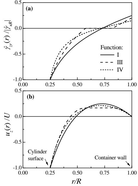
Figure 2. (a) Shear rate and (b) velocity profiles, as a function of the radial coordinate in the annular gap between cylinders. Geometrical characteristics used in calculations are R=0.005 m and \kappa=0.25 . In particular, \Delta\rho=100 kg/m 3 in the case of Function III and 200 kg/m 3 in the case of Function IV. The parameter values of the viscosity functions are reported in the text.
