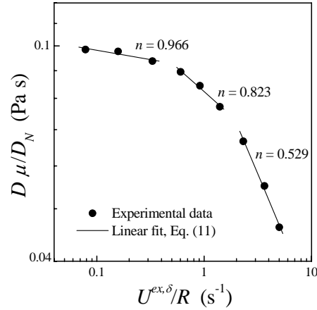
Figure 6. Apparent viscosity as a function of the ratio U/R for a fluid obeying Function IV, with \delta = 0.01 . Symbols are the values obtained from the relative drag force. Lines represent the prediction of Eq. (11) for different intervals of U/R .
