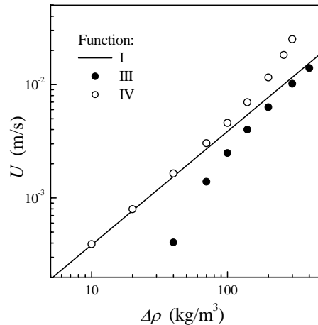
Figure 3. Terminal velocity of the falling cylinder as a function of the density difference, for R = 0.005 m and \kappa = 0.25 . The parameter values are reported in the text. The line representing the Newtonian fluid is obtained from Eq. (A2) with \mu=0.1 Pa s.
