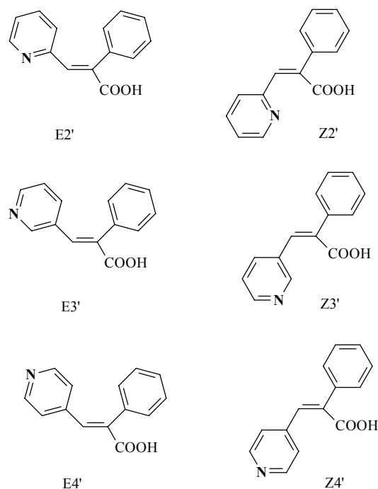
Figure 1. The molecules studied.
