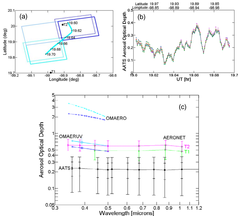
Fig. 12. For the 19 March J31 science flight over the Mexico City urban complex: (a) plan view of the J31 lowest altitude flight track near T2 and intersecting OMI (OMAERUV solid, OMAERO dotted) pixels, with J31 flight track times in UT; (b) AOD measured by AATS along this flight track (wavelength color code as in Fig. 2); (c) AOD spectra retrieved by OMAERO (x symbols with dashed lines), OMAERUV (circles with solid lines), AATS (squares with short dashed line), and AERONET (at T1 and T2).
