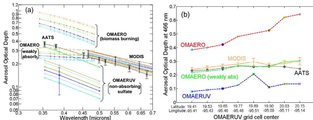
Fig. 5. For 10 March: (a) AOD spectra retrieved by OMAERO (x symbols with dashed lines), OMAERUV (circles with solid lines), MODIS (triangles with solid lines), and AATS (squares with short dashed line). The color scheme is the same as that used in Figs. 2b and 3. The AOD at the primary OMAERUV retrieval wavelength of 388 nm is emphasized with concentric circles. For OMAERUV and MODIS, vertical bars give representative uncertainties. For AATS, vertical bars give the AOD measurement uncertainty (narrow ticks), standard deviation (medium width ticks) and range (wide ticks) along the track. Two sets of OMAERO results are plotted: the archived retrievals that yield biomass-burning aerosol models, and a special run constrained to retrieve only weakly absorbing aerosol models. (b) Variation of AOD at 466 nm as a function of OMAERUV pixel, where AATS and OMI values have been interpolated to 466 nm. Vertical bars on the MODIS data give the range of MODIS retrievals for all MODIS pixels intersecting the OMAERUV pixel.
