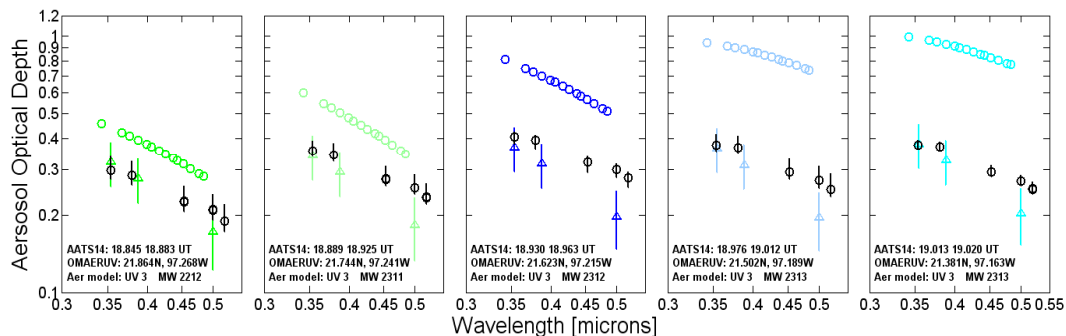
Fig. 8. Comparison of AOD spectra from AATS (black circles with vertical lines showing the range), OMAERO (colored circles), and OMAERUV (triangles with vertical bars giving the expected AOD uncertainty) for the 3 March case study.
