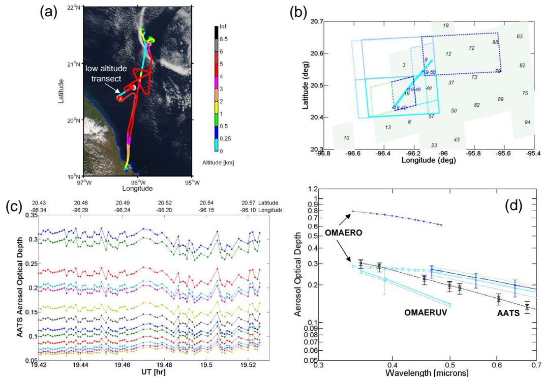
Fig. 9. Case study for 17 March: (a) Aqua-MODIS true color image with color-coded J31 flight track; (b) plan view of the J31 low-altitude flight track and intersecting OMI (OMAERUV solid, OMAERO dotted) and MODIS (dashed) pixels, with all nonzero MODIS cloud percentages; (c) AOD measured by AATS along the low altitude J31 flight track; (d) AOD spectra retrieved by OMAERO (x symbols with dashed lines), OMAERUV (circles with solid lines), and AATS (squares with short dashed line). The color scheme is the same as in (b).
