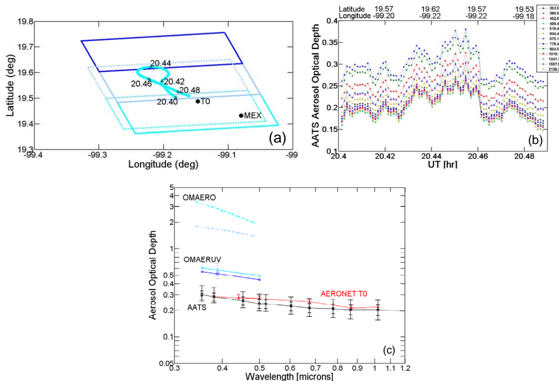
Fig. 13. For the 19 March J31 science flight over the Mexico City urban complex: (a) plan view of the J31 lowest altitude flight track near T0 and intersecting OMI (OMAERUV solid, OMAERO dotted) pixels, with J31 flight track times in UT; (b) AOD measured by AATS along this flight track (wavelength color code as in Fig. 2); (c) AOD spectra retrieved by OMAERO (x symbols with dashed lines), OMAERUV (circles with solid lines), AATS (squares with short dashed line), and AERONET (at T0).
