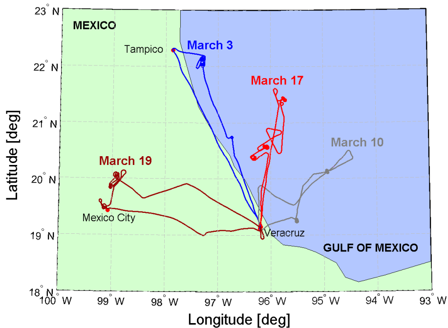
Fig. 1. Map view of the four J31 flight tracks coincident with OMI overpasses during MILAGRO.
