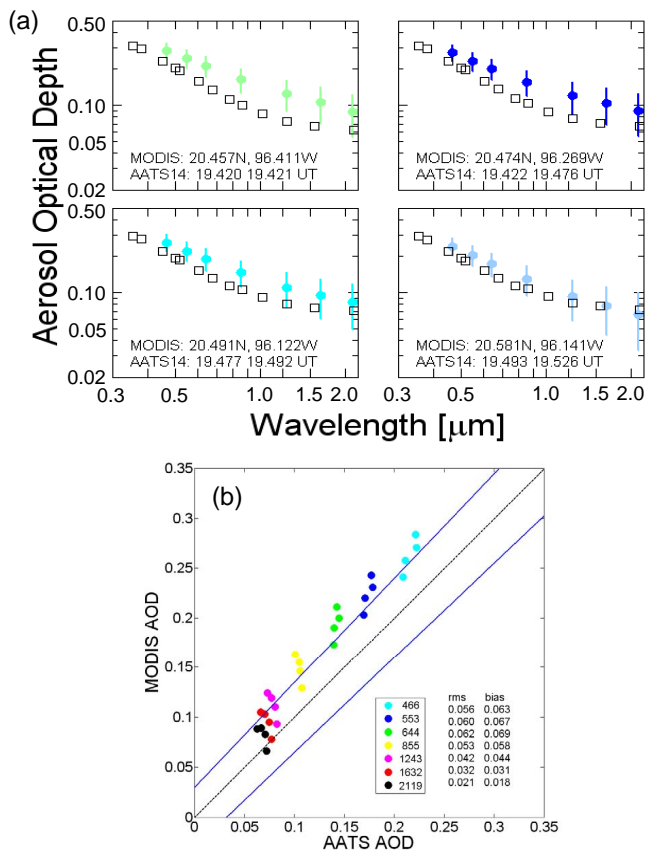
Fig. 10. Case study for 17 March: (a) Comparison of AATS (black squares) and MODIS (colored dots with vertical bars showing estimated uncertainties) AOD spectra within each MODIS pixel; (b) Scatterplot of MODIS vs. AATS AOD, where AATS values have been interpolated to the MODIS wavelengths. The black dashed line gives the one-to-one correspondence, and the two blue lines delineate the expected MODIS AOD uncertainty of \pm(0.03+0.05 \cdot \text{AOD}) .
