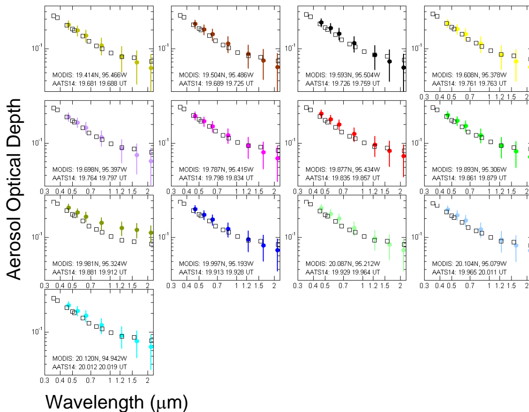
Fig. 3. Comparison of AATS and MODIS AOD spectra within MODIS pixels along the J31 low altitude flight track on 10 March.
