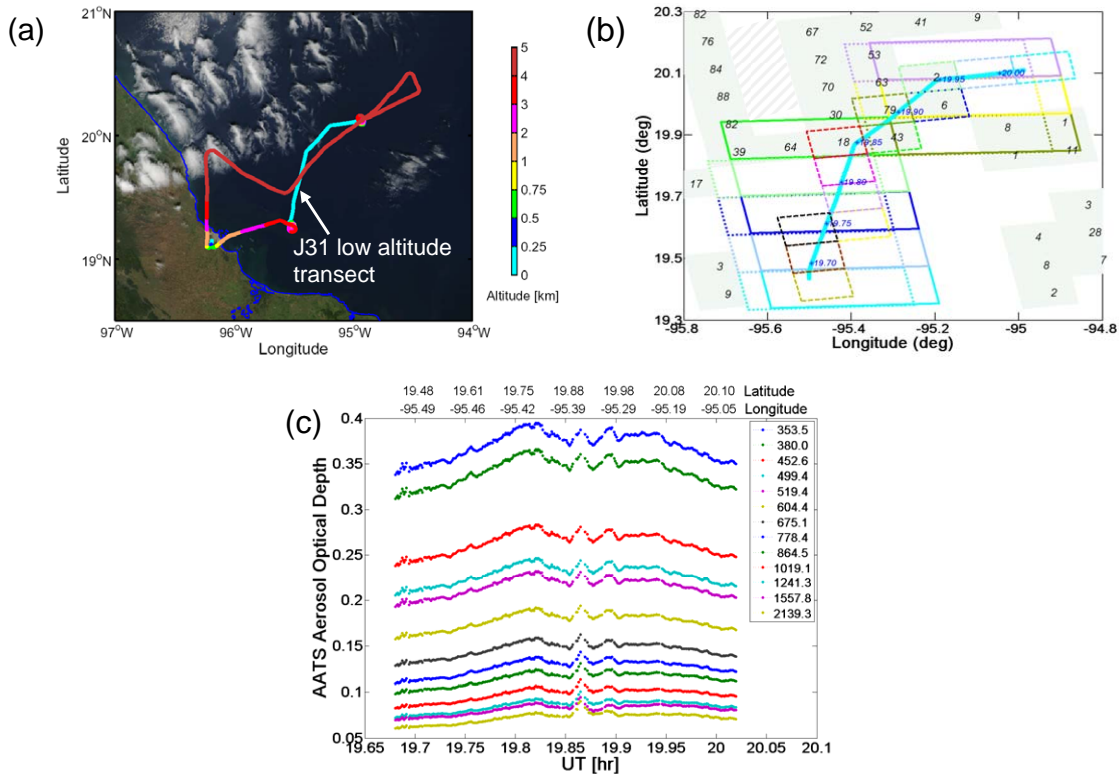
Fig. 2. Case study for 10 March: (a) Aqua-MODIS true color image with superimposed J31 flight track color-coded by altitude; (b) plan view of the J31 low altitude flight track and intersecting OMI (OMAERUV solid, OMAERO dotted) and MODIS (dashed) pixels, with all nonzero MODIS cloud percentages and with times (UT) along the flight track; (c) AOD measured by AATS along the low altitude J31 flight track.
