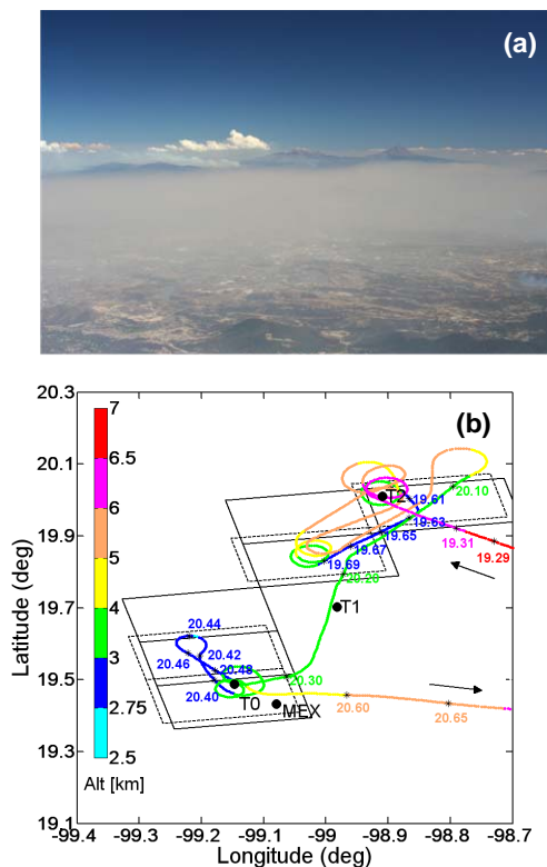
Fig. 11. For the 19 March J31 science flight over the Mexico City urban complex: (a) photo taken looking east from the DC-8 at an altitude of 7000 m at 19:25 UT; (b) plan view of the altitude color-coded J31 low-altitude flight track and intersecting OMI (OMAERUV solid, OMAERO dotted) pixels. Locations of AERONET sites at T0, T1, and T2 are shown, in addition to the Mexico City International Airport (MEX). The two lowest altitude J31 flight legs near T2 and T0 are dark blue; small black asterisks mark location of J31 corresponding to the listed times in UT.
