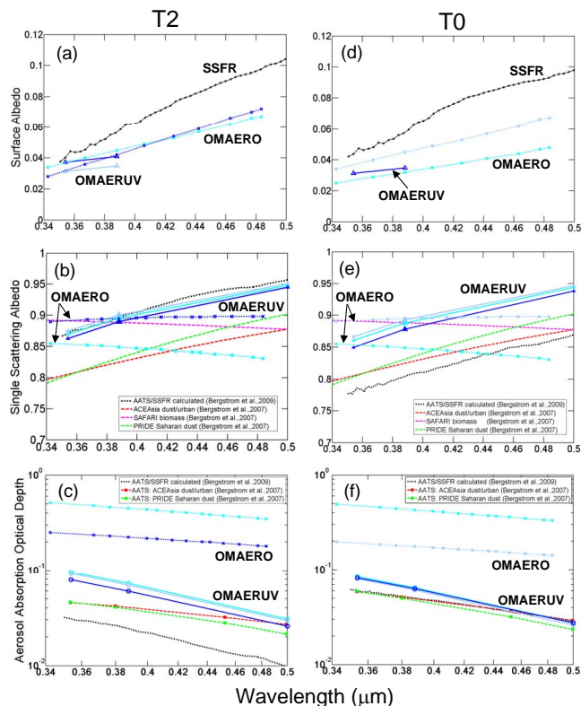
Fig. 14. For AATS and OMI measurements near the T2 (a–c) and T0 (d–f) supersites on 19 March: (a), (d) Surface albedos assumed by the OMI retrieval algorithms and derived from coincident J31 SSFR measurements; (b), (e) Single scattering albedos from the OMI retrievals, from Bergstrom et al. (2009) for T2 and T0, and from Bergstrom et al. (2007) results for ACE Asia dust/urban, SAFARI biomass-burning, and PRIDE Saharan dust aerosol; (c), (f) AAOD derived from the OMI retrievals, and calculated from AATS AODs assuming various Bergstrom et al. (2007, 2009) results (see text for discussion).
