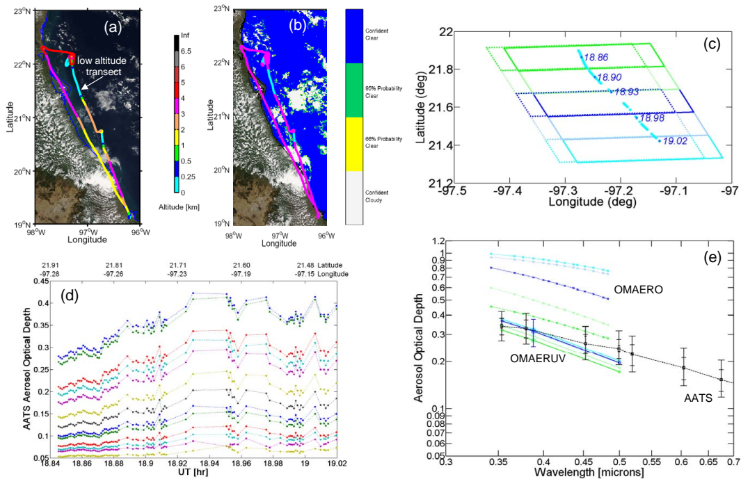
Fig. 7. Case study for 3 March: (a) Aqua MODIS true color image with color-coded J31 flight track; (b) MODIS standard cloud mask product; (c) plan view of the J31 low-altitude flight track and intersecting OMI (OMAERUV solid, OMAERO dotted) pixels, with J31 flight track times; (d) AOD measured by AATS along the low altitude J31 flight track with same color code as in Fig. 2c; (e) AOD spectra retrieved by OMAERO (x symbols with dashed lines), OMAERUV (circles with solid lines), and AATS (squares with short dashed line). The color scheme is the same as in (c). Vertical bars on AATS AODs are described in Fig. 5 caption.
