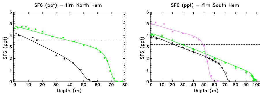
Fig. 12. Comparison of the firn model results (continuous lines) for SF 6 with FIRETRACC and CRYOSTAT data (symbols). Measurements made at UEA are shown as stars, those made at MPI (Sturges et al., 2000; FIRETRACC, 2007) as plus signs. Drilling sites representation: see Fig. 5.
