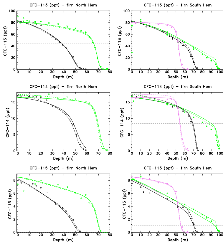
Fig. 10. Comparison of the firn model results with our emission-based scenarios (continuous lines) and the Sturrock et al. (2002) concentration-based mean scenarios (dashed lines) for minor CFCs with FIRETRACC and CRYOSTAT data (symbols). See Fig. 5 for drilling sites and measurement lab. symbols. The Sturrock et al. (2002) trend scenarios were extrapolated from 1997 to 2003 in order to simulate the North GRIP and Berkner firn data.
