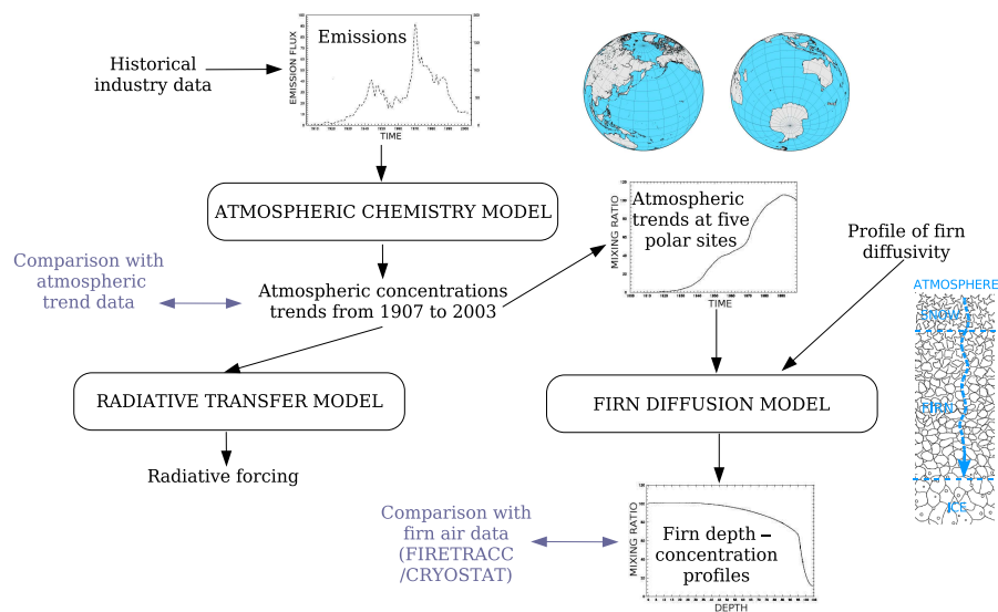
Fig. 1. Combined use of 3 numerical models.
