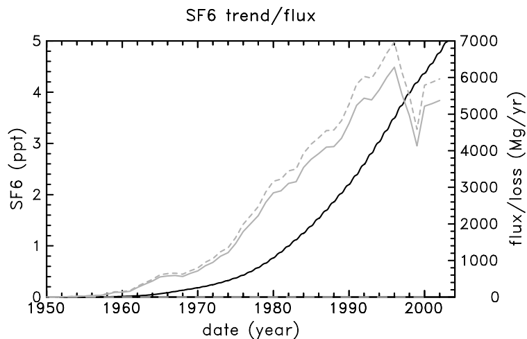
Fig. 13. SF 6 concentration trends at the latitude of Cape Grim (in black) and emission scenarios (in grey) constructed from industrial inventories (continuous line, see Sect.2.1), and corrected to fit the CMDL atmospheric record (dashed line).
