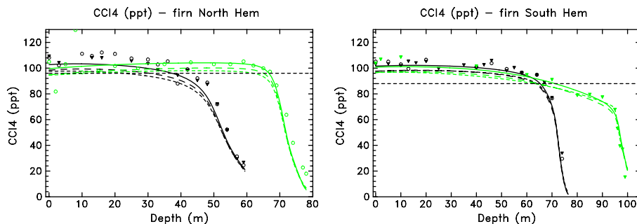
Fig. 11. Comparison of the firn model results with our emission-based scenarios (continuous lines: emissions adjusted to CMDL data, long dashed lines: emissions adjusted to AGAGE data) and the Sturrock et al. (2002) concentration-based mean scenarios (short dashed lines) for \text{CCl}_4 with FIRETRACC and CRYOSTAT data (symbols). See Fig. 5 for drilling sites and measurement lab. symbols. There is no reliable \text{CCl}_4 record at Berkner Island.
