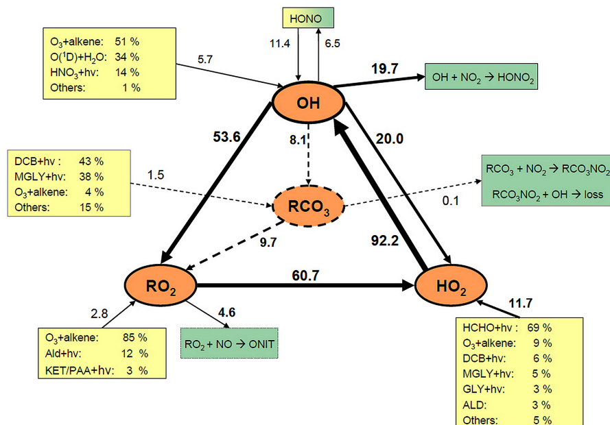
Fig. 8. Rate of production analysis performed for the median campaign measurements from 08:40 a.m. to 06:40 p.m. Initiation, termination and propagation rates are in 10^6 molecule/cm 3 /s. The percentage values represent the contribution of each process to the rate.
