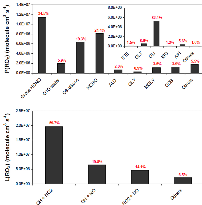
Fig. 7. Model-calculated rates of RO x initiation and termination averaged between 08:40 a.m. and 06:40 p.m. Note that these calculations are based on a gross initiation rate of OH from HONO photolysis. The contribution of HONO photolysis to the total rate of RO x initiation would be smaller on a net basis.
