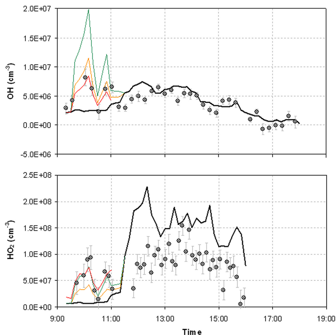
Fig. 4. HO x concentrations observed on March 16 th . Time is CST. Grey circles are individual measurements and error bars are the 1 \sigma precision. Simulations performed using the dataset described in Sect. 3 with additional constraints for MGLY and DCB are displayed by black lines. Orange and green lines represent simulations performed with an additional production of HO 2 in the RACM mechanism for the morning hours (see Sect. 4.3.1). Red lines are simulations performed using an additional production of HO 2 and a reaction rate for HO 2 +NO divided by a factor 2.5 (see Sect. 4.3.1). For 16 March, additional production rates of HO 2 are 1.1 \times 10^8 , 2.2 \times 10^8 and 0.7 \times 10^8 molecule/cm 3 /s for the orange, green and red lines, respectively.
