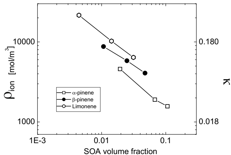
Fig. 12. Values of hygroscopicity versus the SOA-volume-fraction for SOA produced from different precursors, derived for data given in VanReken et al. (2005) and assuming \sigma_{s/a}=72 mN/m.
