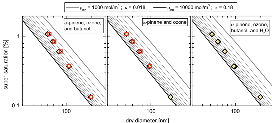
Fig. 8. Activation of for three different types of SOA particles, measured with the DMT-CCNc. Different symbols result from measurements that were done on different days for similar experimental conditions. Grey lines are contour lines indicating the relation between dry particle diameter and the super-saturation needed for activation for constant hygroscopicity.
