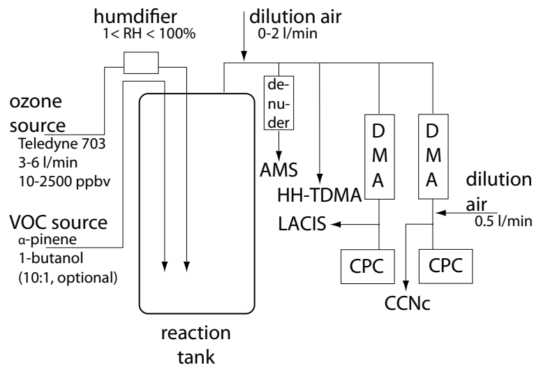
Fig. 1. Schematic of the experimental setup for the measurements.
