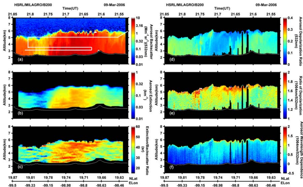
Fig. 3. Time-height plots of 532 nm aerosol backscatter (a) , 532 nm aerosol extinction (b) , 532 nm lidar ratio (c) , aerosol depolarization ratio at 532 nm (d) , ratio of the 1064 nm depolarization ratio to the 532 nm depolarization ratio (e) , and the aerosol backscatter wavelength dependence (f) . The thick white line in aerosol backscatter indicates the altitude that the G-1 aircraft flew making in situ measurements along this flight track. Note that the top axis is the HSRL time and only the G 1 longitude is represented here; the G-1 flew this flight track within an hour of the HSRL times (21:08 UTC to 22:06 UTC).
