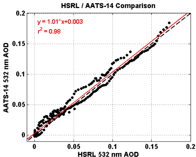
Fig. 10. Comparison of 532 nm AOD from HSRL and AATS-14 for all three profiles acquired on 10, 12, and 15 March 2006 with the bilinear regression in red and the one to one line in black (dashed).
