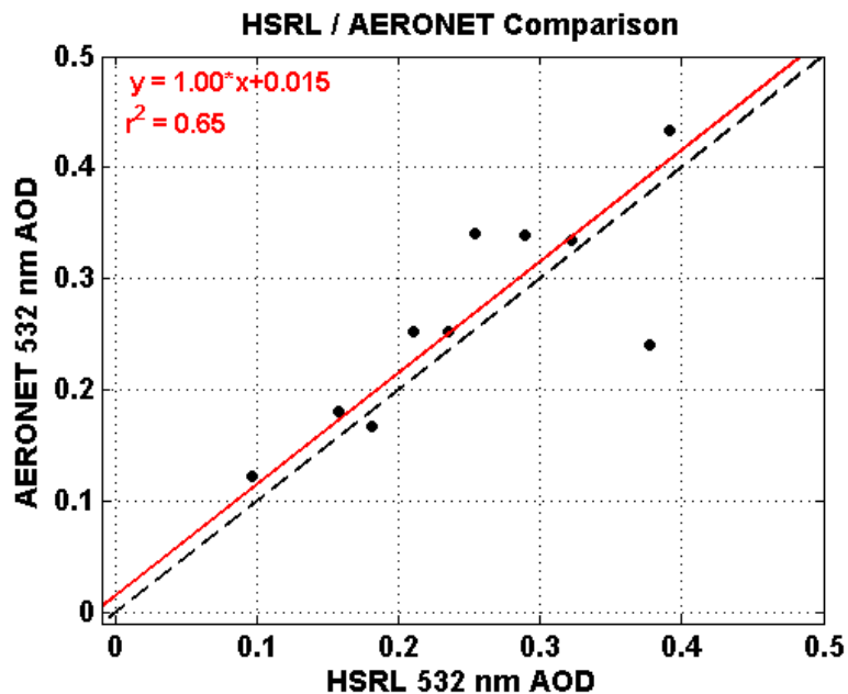
Fig. 12. Comparison of 532 nm AOD from HSRL and AERONET (all stations) using 1 h and 10 km as the criteria for coincidence. The black dashed line is the one to one line and the red line is the bilinear regression.
