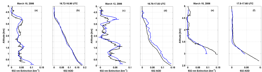
Fig. 8. Profile comparisons of HSRL and AATS aerosol extinction at 532 nm ( a, c, e ) and differential AOD at 532 nm ( b, d, f ). These are from three spirals on 10 March 2006 ( a, b ), 12 March ( c, d ) and 15 March 2006 ( e, f ). On 15 March 2006 the lower limit is 2.5 km because this spiral was over vertically varying terrain with surface altitudes up to 2.6 km. Note that the HSRL 532 nm AOD profiles extend closer to the ground than the HSRL extinction because of the extrapolation. Random uncertainty for both HSRL is plotted for 532 nm extinction; corresponding AATS extinction uncertainties are described in the text.
