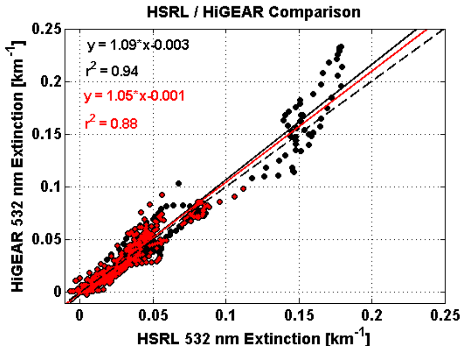
Fig. 7. Comparison of 532 nm extinction (black circles) from HSRL and HiGEAR for all four profiles acquired on three days: 10, 28, and 29 March 2006. Data points corresponding to relative humidity less than 65% are indicated with a smaller red circle. Black and red lines are the bilinear regression for all data and data with relative humidity less than 65%, respectively. The black dashed line is a one-to-one line.
