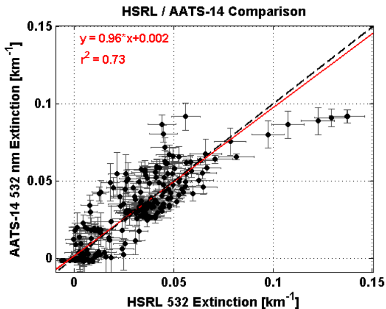
Fig. 9. Comparison of 532 nm extinction from HSRL and AATS 14 for all three profiles acquired on 10, 12, and 15 March 2006. Red and black (dashed) lines indicate the bilinear regression and the one to one line, respectively.
