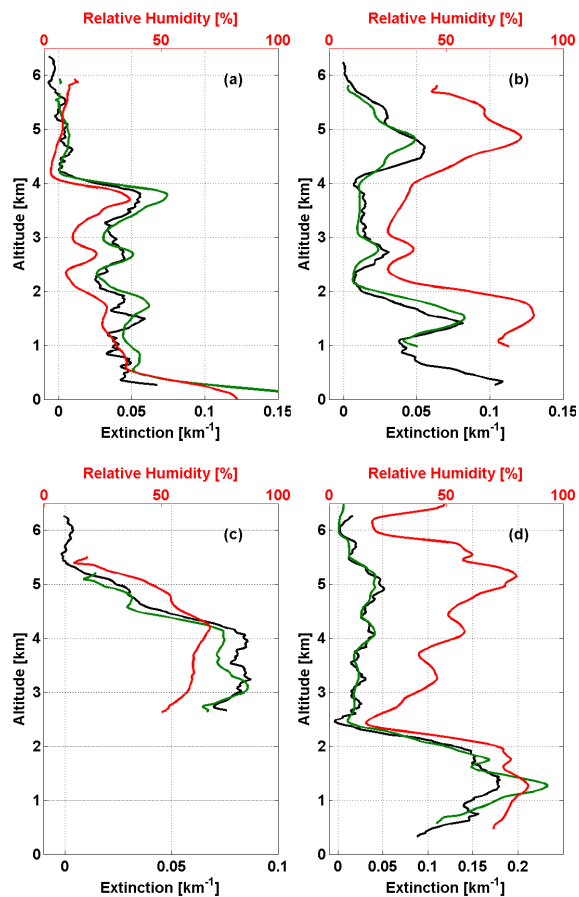
Fig. 6. Vertical profiles of HSRL and HiGEAR derived extinction 10 March 2006 (a) 28 March 2006 (b) 29 March 2006 (1st spiral) (c) 28 March 2006 (2nd spiral) (d) . The relative humidity from the C-130 is shown in red.
