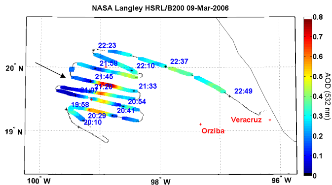
Fig. 2. Flight track maps of (a) aerosol backscatter coefficient (only every other leg is plotted for clarity) and (b) aerosol optical depth on 9 March 2006 over the Mexico City basin. The black arrows indicate the leg that is coordinated with the G-1.
