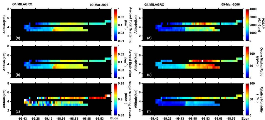
Fig. 4. A subset of measurements from the G-1 aircraft including aerosol total scattering (a) , aerosol extinction (b) , single scattering albedo (c) , aerosol number density (0.1–3 \mu\text{m} ) (d) , ozone mixing ratio (e) , and relative humidity (f) .
