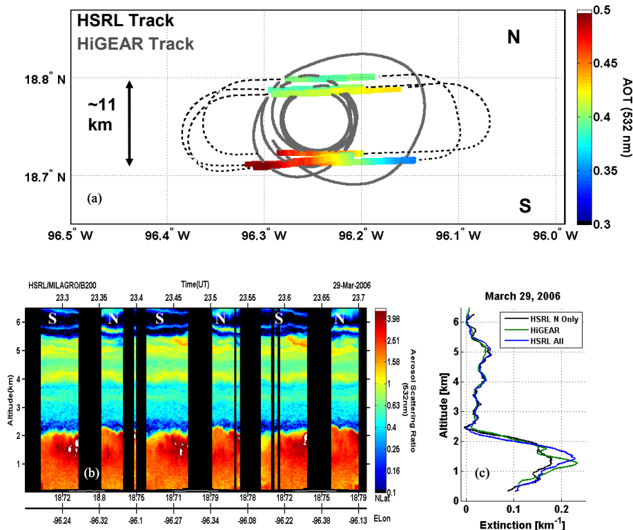
Fig. 5. (a) 29 March 2006 coincident HSRL (black dashed) and HiGEAR (grey) flight tracks with HSRL AOD shown along the straight legs, (b) backscatter ratio time-height plot over the same time period with the north and south legs indicated, (c) average extinction profile from HiGEAR and HSRL, with HSRL data averaged over the northern legs only and also over both the northern and southern legs.
