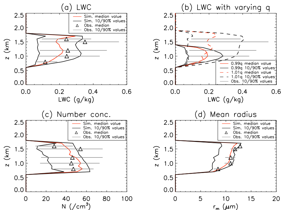
Fig. 2. Vertical profiles of the simulated (red) and observed (triangles) median values of (a) LWC, (c) droplet number concentration and (d) r_m of the base case. (b) shows vertical profiles of the median values of the LWC of the simulations with 99% and 101% of the specific humidity (respectively red solid and broken lines). Simulated 10 and 90% values are depicted with solid (broken) black lines. The horizontal grey lines through the triangles depict the observed range between the 10% and the 90% values.
