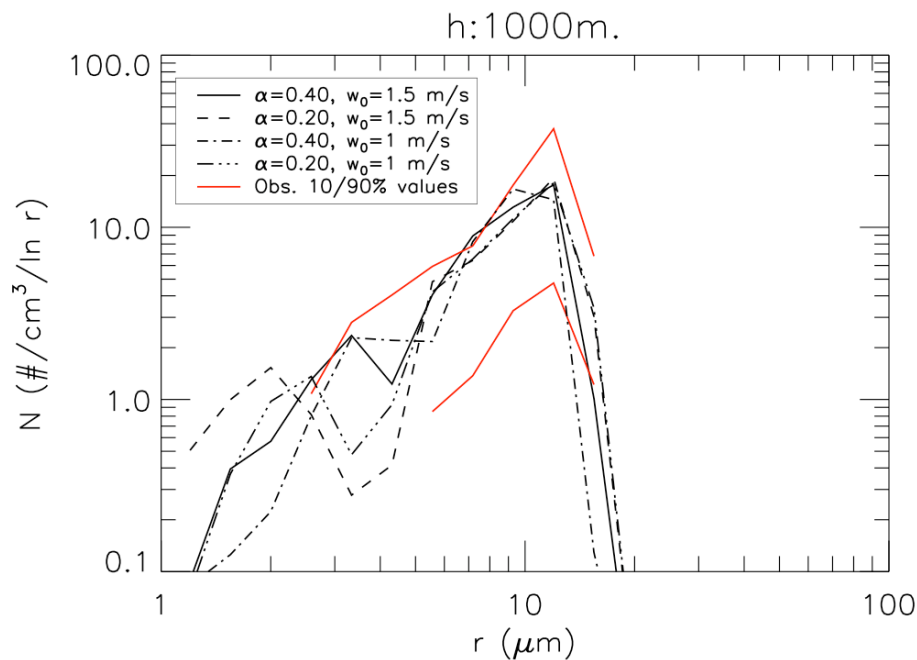
Fig. 6. Time averaged cloud droplet size distributions at 1000 m height for four simulations: base case (solid black line), \alpha=0.2 and w_0=1.5 m/s (dashed line), \alpha=0.4 and w_0=1 m/s (dot-dashed line) and \alpha=0.2 and w_0=1 m/s (dot-dot-dashed-line). In red are the 10 and 90% values from the observations.
