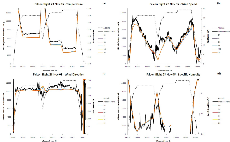
Fig. 5. Same as Fig. 4 but for the Falcon data.
