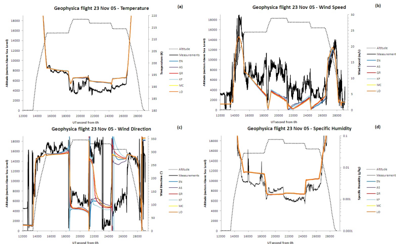
Fig. 4. Comparison between the Geophysica meteorological data and the six model simulations. (a) Temperature (K), (b) horizontal wind speed ( \text{m s}^{-1} ), (c) wind direction ( ^{\circ} ) and (d) specific humidity ( \text{g kg}^{-1} ). The black lines are for the aircraft measurements and the coloured lines for the model results. The dashed line is the model altitude in m.
