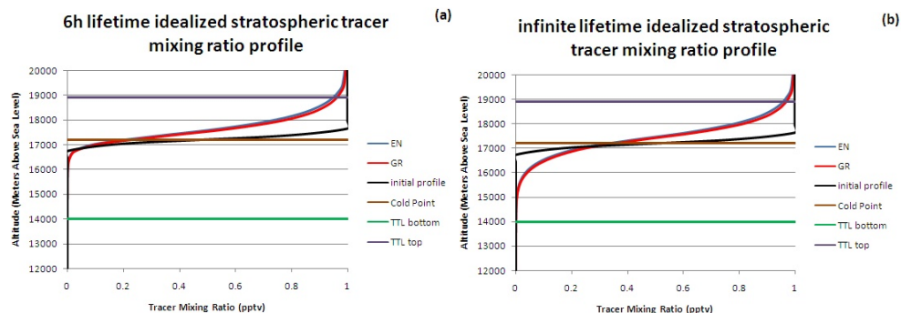
Fig. 10. Same as Fig. 6 but for Tracer 3 and 4 (stratospheric tracers). The dark line is the mean vertical profile at the initial time of the simulation.
