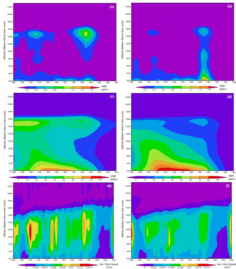
Fig. 8. Meridian mean of Tracer 1 from EN (a) and GR (b) simulations. (c) and (d) are respectively the same plots but for Tracer 2; and (e) and (f) for vertical velocity. The mean is calculated from the one month period using the 3-hourly outputs.
