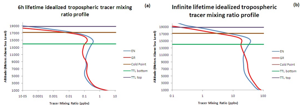
Fig. 6. Volumetric tracer mixing ratio profiles (in ppbv) averaged over the model domain and over the one month simulation period using 3-hourly model outputs for (a) Tracer 1 and (b) Tracer 2. The blue lines correspond to the EN simulation and the red lines to the GR simulation.
