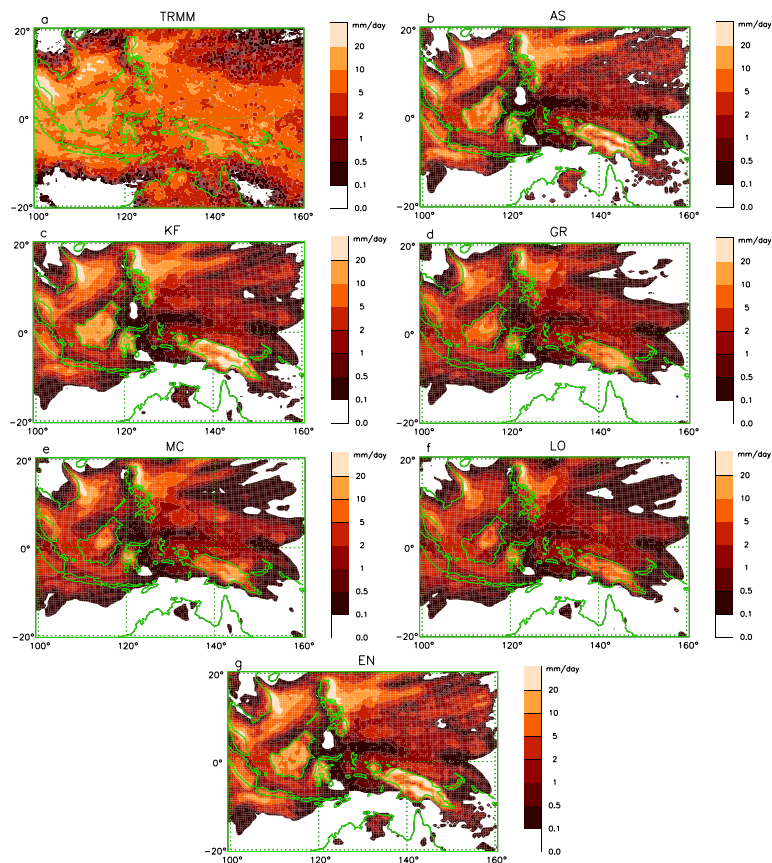
Fig. 2. Daily mean surface rainrate in \text{mm day}^{-1} from 15 November 2005 to 15 December 2005 for (a) TRMM and the model simulations using (b) Arakawa-Schubert, (c) Kain-Fritsch, (d) Grell, (e) Moisture Convergence, (f) Low Omega, (g) Ensemble.
