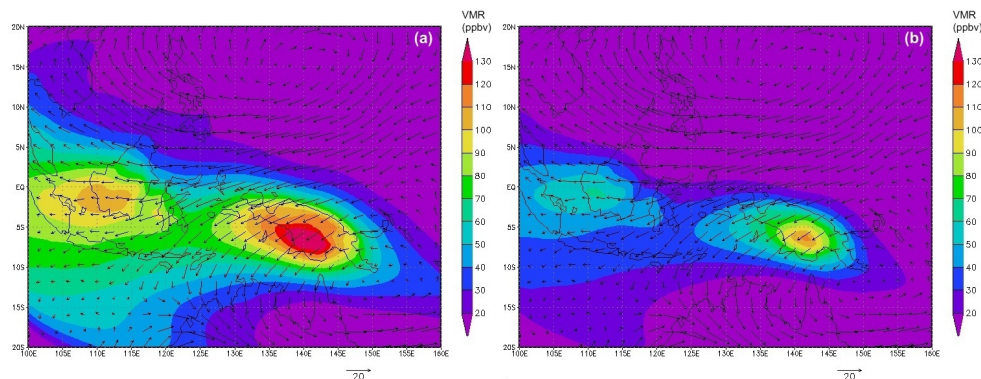
Fig. 9. 15 km height mean of Tracer 2 from EN simulation (a) and GR simulation (b). Wind vector are over plotted. The mean is calculated from the one month period using the 3-hourly outputs.
