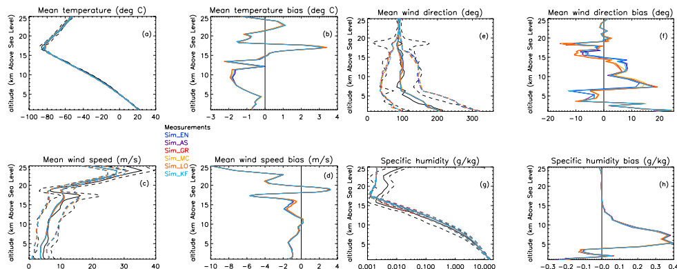
Fig. 3. Comparison between the Manus radiosounding data and the six model simulations: (a and b) for temperature, (c and d) for horizontal wind speed and (e and f) wind direction, (g and h) for specific humidity. Left panels display the mean (solid line) and standard deviation (dashed line) and right panels the mean bias (model minus observation). Black lines are for the radiosounding data and colored lines for the model simulations. The radiosounding data are averaged over the model vertical levels.
