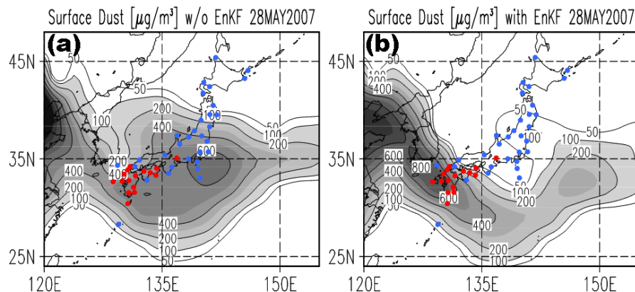
Fig. 5. Comparison of simulated surface dust concentrations on 28 May 2007 (contours and gray shades; daily mean) and the weather stations (red circles) that observed aeolian dust events, so-called Kosa, on the same day (plotted only in Japan). Blue circles indicate the weather stations that did not observe any aeolian dust events on the day. (a) Reference model run without assimilation and (b) 4D-LETKF assimilation results.
