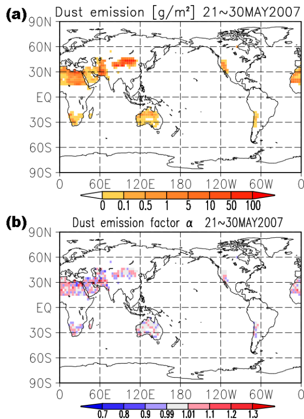
Fig. 2. (a) Simulated dust emission intensity in MASINGAR without assimilation from 21 to 30 May 2007; all 10 size bins are accumulated. (b) Dust emission factor \alpha for each grid point estimated by 4D-LETKF assimilation; averaged from 21 to 30 May 2007 across all 10 size bins.
