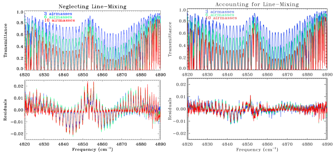
Fig. 8. Residuals obtained from fits of ground-based atmospheric solar-absorption spectra in Band#1 for various airmasses. The panels on the left and right hand sides display results obtained without and with the inclusion of LM, respectively.
