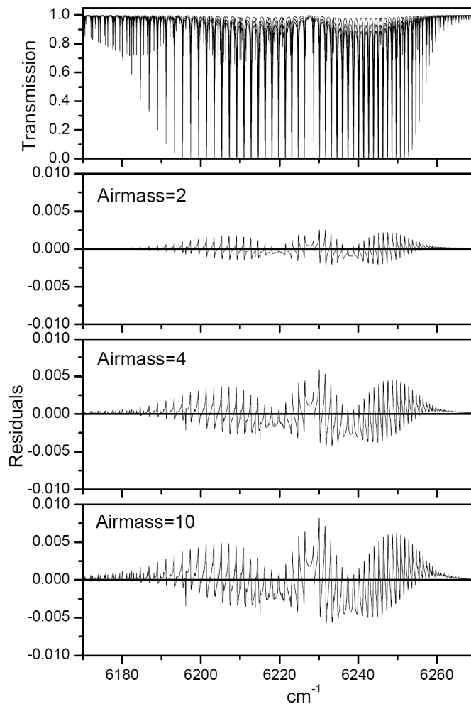
Fig. 7. Same as Fig. 6 but for Band#2.
