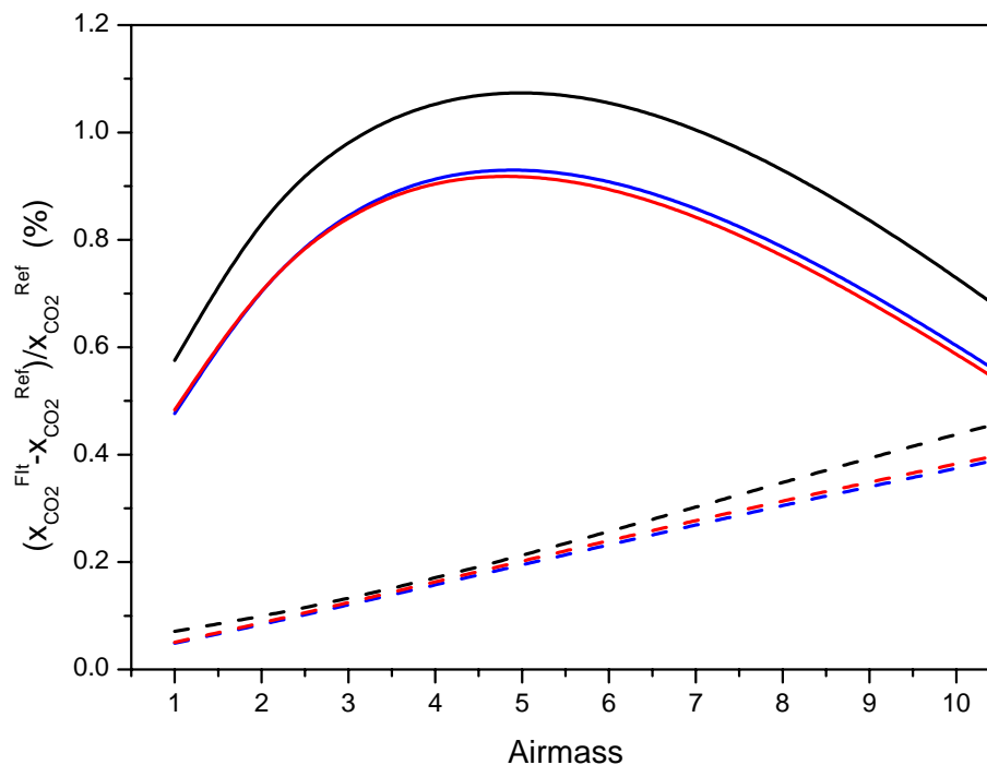
Fig. 3. Influence of the spectral resolution on the errors on CO 2 vmr retrieved neglecting line-mixing effects. The results are for MOPD's of 2 cm (—), 10 cm (—) and 50 cm (—). The upper (full lines) and lower (dashed lines) sets of three curves refer to Band#1 (4765–4915 cm -1 ) and Band#2 (6160–6270 cm -1 ), respectively.
