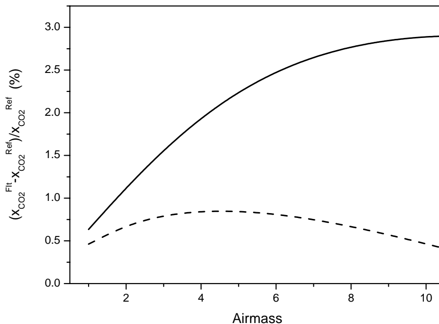
Fig. 5. Relative errors, induced by neglecting LM, on the CO 2 vmr deduced from fits of spectra with a 50 cm MOPD for various airmasses. --- and — are values obtained in Band#1 by fitting the full region between 4765 and 4915 cm -1 and by restricting the fits to the 4820–4890 cm -1 interval, respectively.
