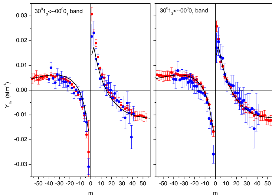
Fig. 1. Comparison of room temperature CO 2 -air first order LM coefficients from the theoretical database of Niro et al. (2005c) (—) with experimental values obtained from multispectrum fits of laboratory spectra in Refs. (Malathy Devi et al., 2007a, b) (•), and (Predoi-Cross et al., 2007) (•). Values are plotted vs. the rotational quantum number m ( m = -J_i for P lines, m = J_i + 1 for R lines) and the error bars on these plots correspond to the one standard deviations given in Malathy Devi et al. (2007a, b) and Predoi-Cross et al. (2007) multiplied by 2 in order to represent the full confidence interval.
