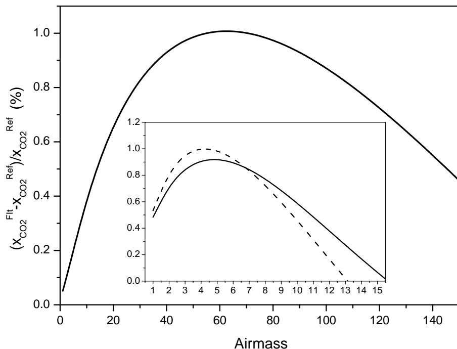
Fig. 4. Relative errors on the \text{CO}_2 vmrs deduced from fits, neglecting line-mixing effects, of spectra with a 50 cm MOPD for various airmasses. The main plot gives results obtained in Band#2. In the insert can be compared results obtained in Band#1 (—) with those obtained in Band#2 (---) after multiplying the Band#2 line intensities by 15.
