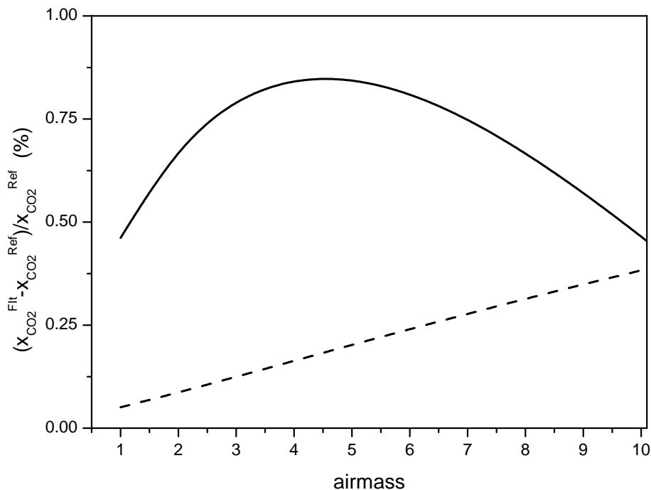
Fig. 2. Relative errors, induced by neglecting LM, on the CO 2 vmrs deduced from fits of spectra with a 50 cm MOPD for various airmasses. The CO 2 vmr and a linear 100% transmission have been adjusted. — and --- are values obtained in Band#1 (4765–4915 cm -1 ) and Band#2 (6160–6270 cm -1 ), respectively.
