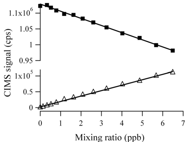
Fig. 3. Sample CIMS calibration using 13 C-labeled acetone (Ac). Squares: sum of \text{H}^+(\text{H}_2\text{O})_n ion counts. Triangles: sum of ion counts corresponding to \text{AcH}^+ , \text{AcH}^+\cdot\text{H}_2\text{O} , \text{AcH}^+\cdot(\text{H}_2\text{O})_2 , and \text{AcH}^+\cdot(\text{H}_2\text{O})_3 . The estimated detection limit for Ac ( \text{signal}=3\sigma_{\text{noise}} ) is 0.01 ppb.
