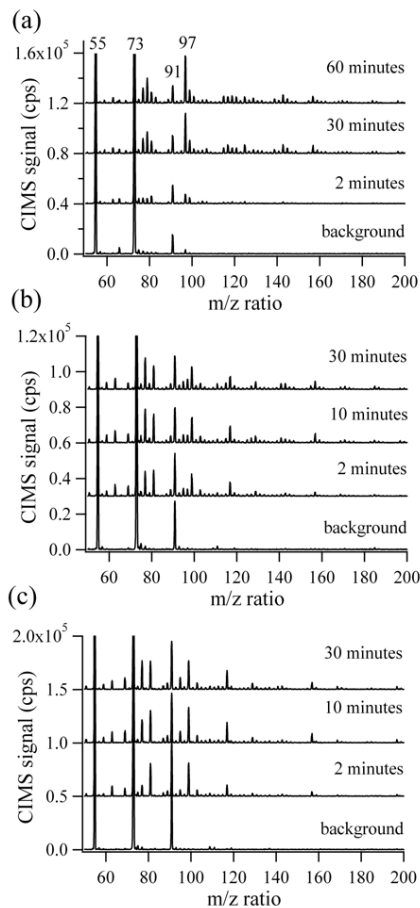
Fig. 4. Representative CIMS spectra of limonene photodegradation products observed after exposure of SOA samples to 290 nm radiation for the specified periods of time. Background spectra were taken immediately before the exposure. Data are presented for SOA prepared with (a) 300 ppm O 3 ; (b) 1 ppm O 3 ; (c) 100 ppb O 3 under the conditions specified in Table 1. The spectra are offset for clarity.
