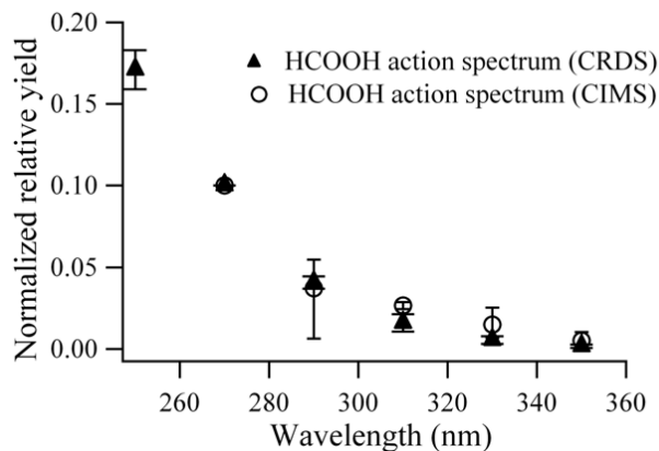
Fig. 10. Comparison of HC(O)OH action spectra recorded with the CIMS instrument and with the CRDS instrument for SOA prepared under high concentration conditions.
