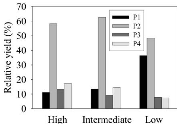
Fig. 12. Distribution of products P1-P4 resulting from kinetic simulations of mechanism in Table 2 using the initial ozone and limonene concentrations listed in Table 1.
