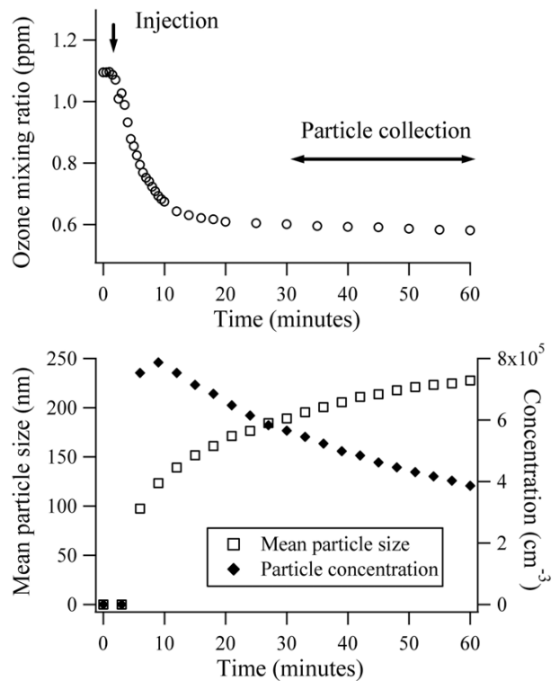
Fig. 1. Concentrations of particles and ozone in the chamber during a typical SOA synthesis.
