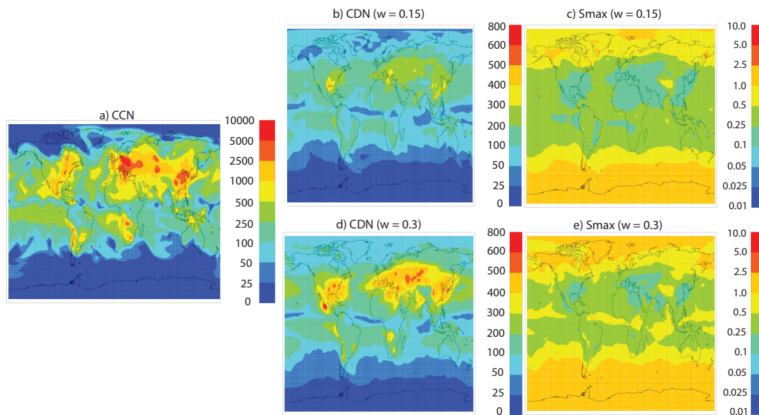
Fig. 1. (a) Global fields of CCN at 0.2% supersaturation ( \text{cm}^{-3} ); (b) CDN concentration ( \text{cm}^{-3} ) predicted using NS03 and an updraft velocity ( w ) of 0.15 \text{ m s}^{-1} ; (c) Maximum supersaturation predicted ( w=0.15 ); (d) and (e) are the same as (b) and (c) but for an updraft of 0.3 \text{ m s}^{-1} . The figures show monthly mean field for October 2001 and an altitude of 920 hPa.
