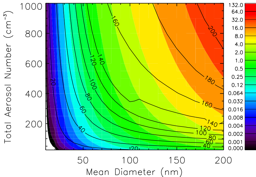
Fig. 5. CDN ( \text{cm}^{-3} ) calculated for a range of lognormal ammonium sulfate aerosol distributions ( \sigma=1.8 ) with an updraft velocity of 0.15 \text{ m s}^{-1} , coloured contours indicate aerosol mass ( \mu\text{g m}^{-3} ).
