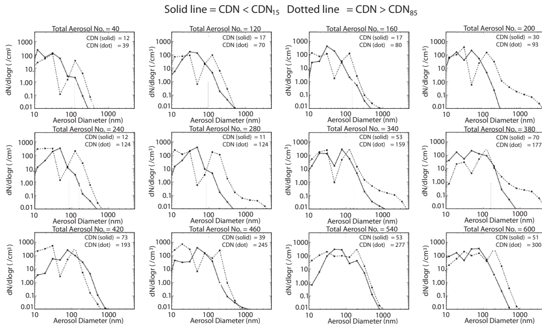
Fig. 3. Aerosol number distributions for a range of total aerosol number concentrations ( D_p > 50 nm), see plot titles for details. The average aerosol number distributions leading to a CDN that is (i) smaller than the 15th percentile ( CDN_{15} ) (solid line) and (ii) larger than the 85th percentile ( CDN_{85} ) (dotted line) are shown.
