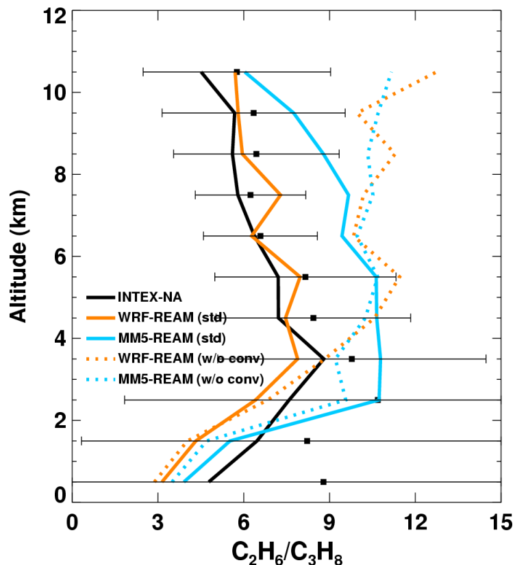
Fig. 3. Observed and simulated vertical profiles of median \text{C}_2\text{H}_6/\text{C}_3\text{H}_8 ratios in the outflow regions over the Western North Atlantic. Black squares show the observed means at 1-km interval. The horizontal bars show the standard deviations. “std” denotes the standard simulation. “w/o conv” denotes the simulation where convective transport is turned off.
