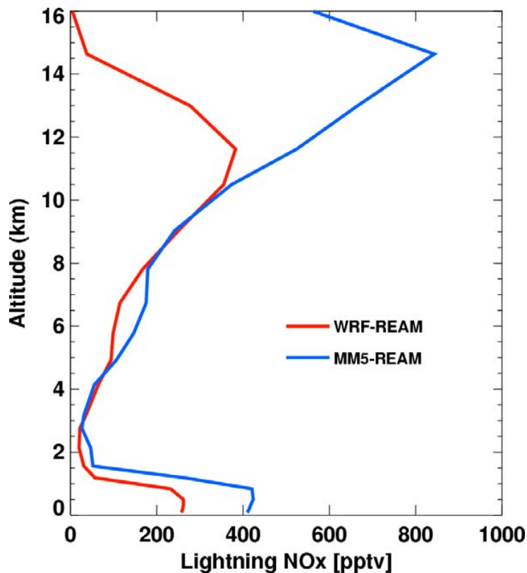
Fig. 5. Mean lightning \text{NO}_x mixing ratio profiles in WRF-REAM and MM5-REAM for July and August 2004 averaged over North America.
