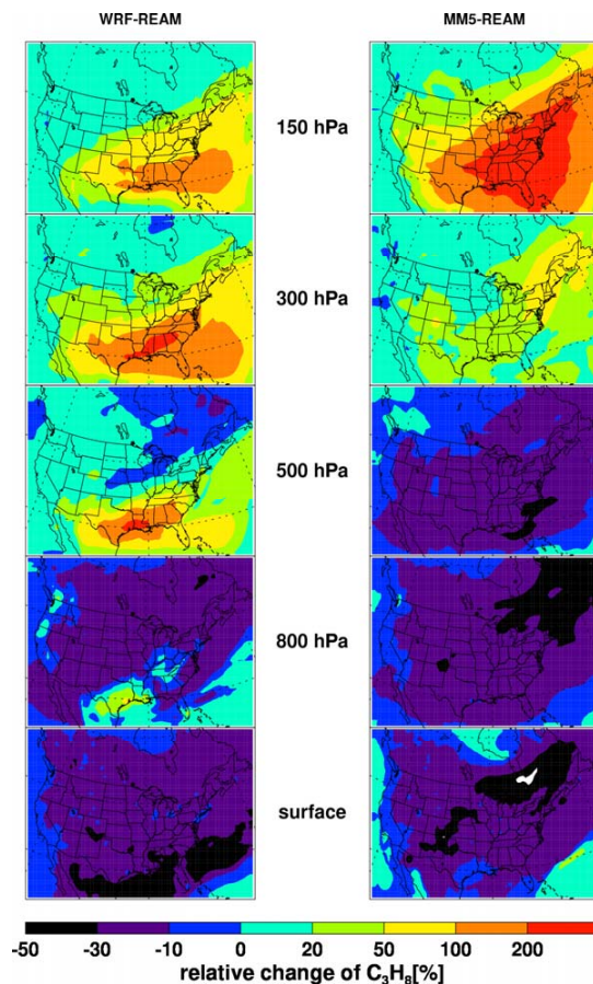
Fig. 2. Percentage changes of \text{C}_3\text{H}_8 in the standard model simulations from the model simulations without convective transport for July and August 2004 at the surface, and 150, 300, 500, and 800 hPa. Results for WRF-REAM and MM5-REAM are shown.
