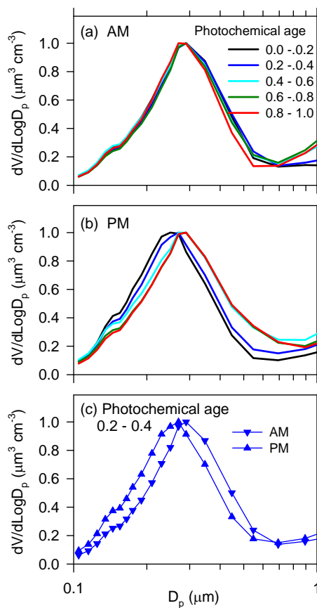
Fig. 7. PCASP volume size distribution, dV/d\text{Log}D , for (a) AM and (b) PM portions of urban data set according to photochemical age with an AM-PM comparison in panel (c) . Same format as Fig. 6.
