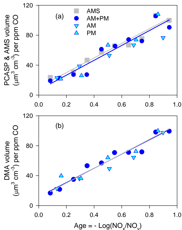
Fig. 2. Dependence of aerosol volume (in excess of background) per ppm of urban CO (in excess of background) on photochemical age. Each data point is the reduced major axis slope from a linear regression of aerosol volume vs. CO. (a) PCASP and AMS volume per CO as a function of photochemical age. Straight lines are linear least squares fit to the AM+PM data points for PCASP and AMS volumes. (b) DMA volume per CO as a function of photochemical age. Straight lines are linear least squares fit to the AM+PM data points for DMA volume and for comparison the AMS linear fit shown in panel a which partially obscures the DMA fit.
