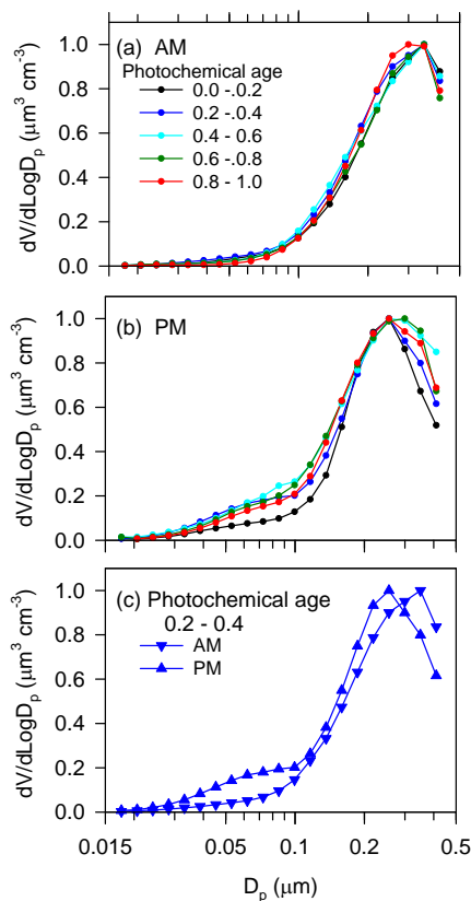
Fig. 6. DMA volume size distributions, dV/d\text{Log}D_p , for (a) AM and (b) PM portions of urban data set according to photochemical age. In panel (c) , AM and PM spectra are compared for the photochemical age range, -\text{Log}(\text{NO}_x/\text{NO}_y) between 0.2 and 0.4. All spectra are normalized to have a peak value of one. Before normalization, spectra differ in magnitude due to dilution and to the addition of condensable species.
