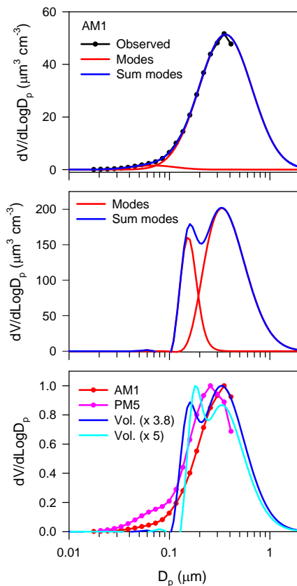
Fig. 10. Volume size spectra showing effects of condensation growth. (a) Observed young DMA spectra (AM1) and a two log normal fit. (b) Fitted log normals after volume of AM1 has increased by a factor of 3.8 by condensation growth mechanism. (c) Observed DMA spectra (AM1 and PM5) compared with calculated spectra after AM1 has grown by a factor of 3.8 and 5. Peak heights normalized to unity.
