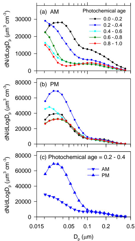
Fig. 9. DMA number size distribution, dN/d\text{Log}D_p , for (a) AM and (b) PM portions of urban data set according to photochemical age with an AM-PM comparison in panel (c). Spectra have not been normalized.
