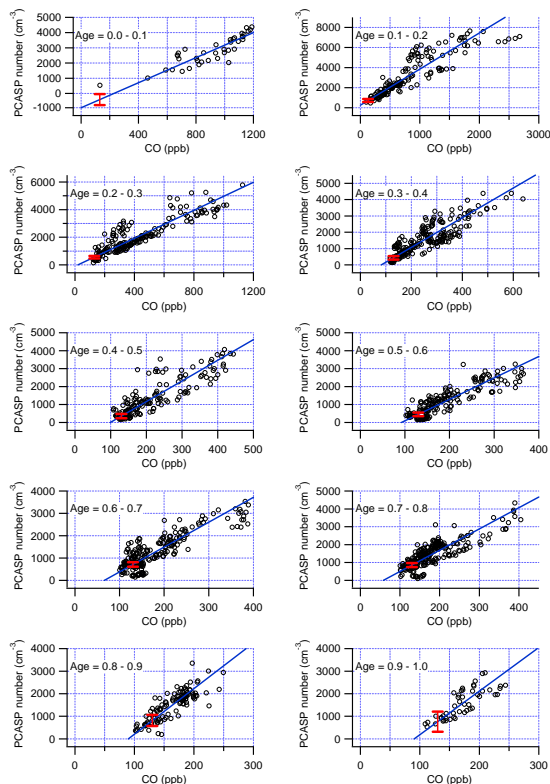
Fig. 5. Scatter plots of PCASP number concentration in the size range 0.1\text{--}0.5\ \mu\text{m} vs. CO concentration. Data set has been split into 10 bins, each spanning 0.1 unit of photochemical age ( -\log_{10}[\text{NO}_x]/[\text{NO}_y] ) as indicated on plots. Each data point represents a 10 s measurement period in the urban plume data set. Blue lines are reduced major axis linear least squares regression fits to data points. Red line shows value and one sigma uncertainty in [Aerosol] at \text{CO}=130\ \text{ppb} .
