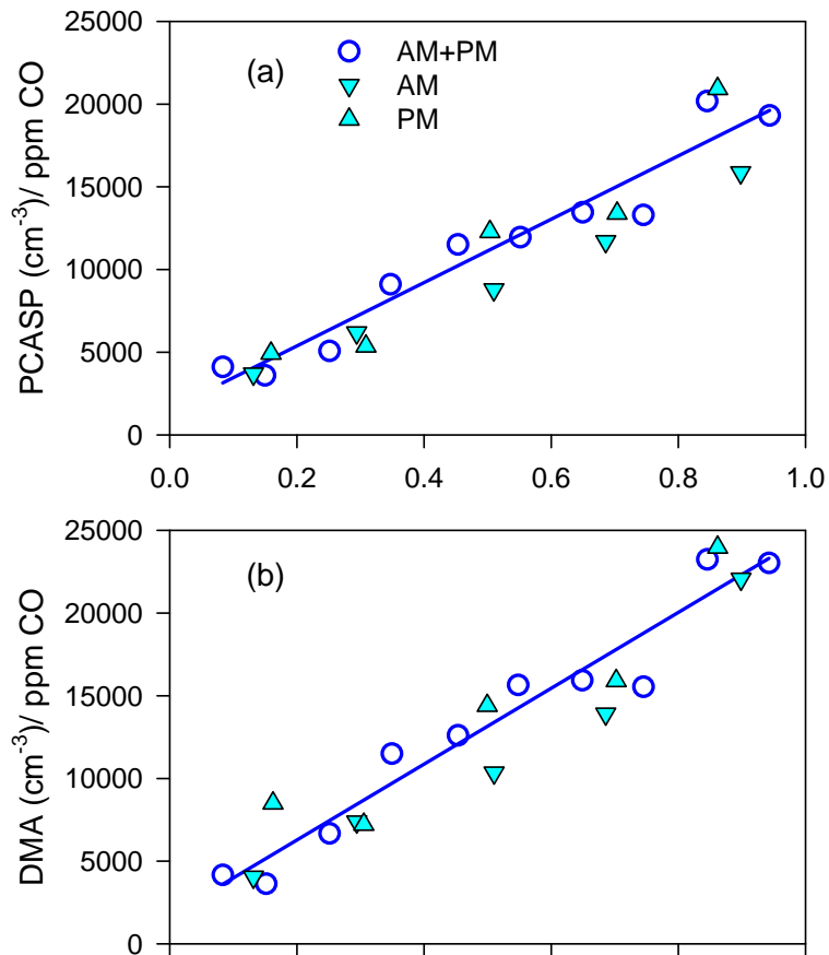
Fig. 4. Data points are slopes of reduced major axis regression of (a) PCASP and (b) DMA number concentration plotted as a function of photochemical age. Same format as Fig. 2.
