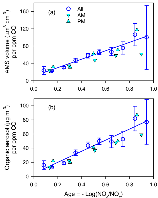
Fig. 3. Data points are slopes from reduced major axis regression of (a) AMS volume and (b) Organic aerosol concentration vs. CO plotted as a function of photochemical age. Error bars are 2\sigma , calculated from \chi^2 of the regressions (Press et al., 1986). Graphs show linear least squares fit to the AM+PM (total) data points for (a) AMS volume and (b) Organic concentration.
