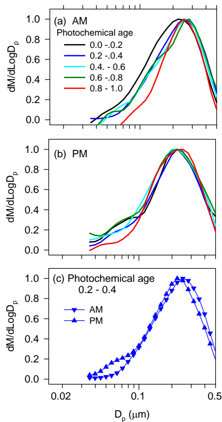
Fig. 8. AMS organic concentration size distribution, dM/d\text{Log}D_p , for (a) AM and (b) PM portions of urban data set according to photochemical age with an AM-PM comparison in panel (c) . Same format as Fig. 6.
