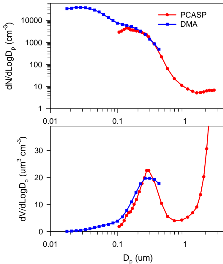
Fig. 1. (a) Aerosol number and (b) volume size distribution measured by the PCASP and DMA for the urban data set. Symbols indicate the geometric mean of size-bin boundaries.
