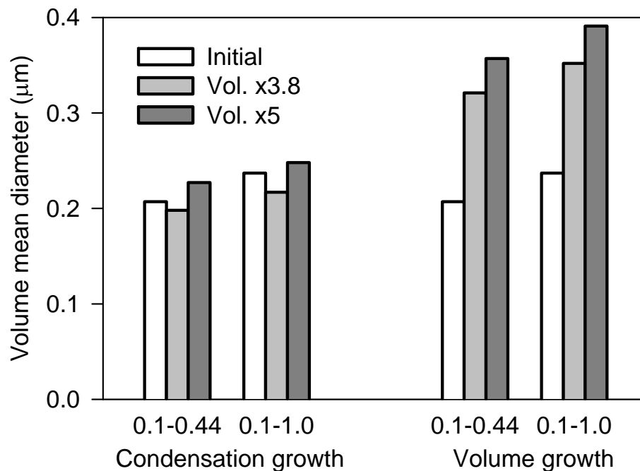
Fig. 12. Volume mean diameter of initial aerosol and that produced after a 3.8 and 5 fold increase in volume by either a condensation or volume growth mechanism. VMD is calculated over 2 size ranges: 0.1–0.44 \mu\text{m} and 0.1–1.0 \mu\text{m} .
