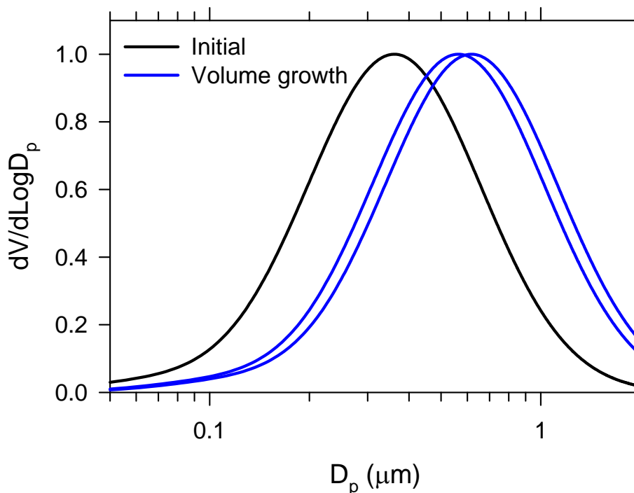
Fig. 11. An initial volume size distribution and size distributions that result from a 3.8 and 5 fold increase in volume by a volume growth mechanism. Spectra are normalized to have the same peak height. The initial distribution is a 2 component log normal fit to the DMA AM1 spectrum (see Fig. 10a). The peak of dV/d\text{Log}D_p is initially at D_p=0.36\ \mu\text{m} and increases to 0.57 and 0.62\ \mu\text{m} after growth. The fractional increase in D_p is 3.8^{1/3} and 5^{1/3} , respectively.
