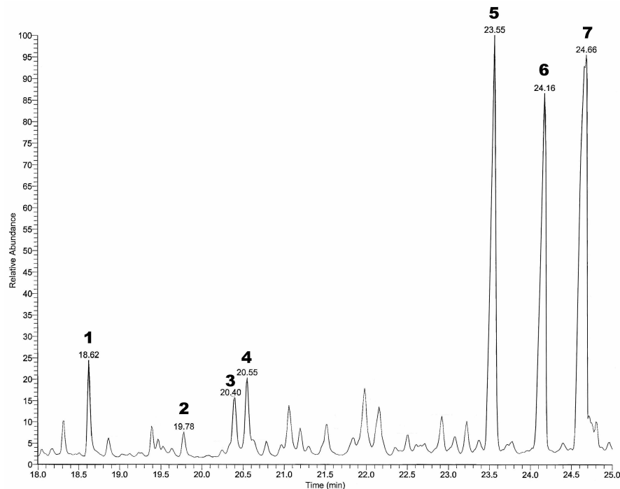
Fig. 3. Total ion chromatogram of filter extract of isoprene SOA formed in the absence of \text{NO}_x from Experiment 4. Identifications: (1) 2-MGA; (2) cis -2-methyl-1,3,4-trihydroxy-1-butene; (3) 2-methyl-2,3,4-trihydroxy-1-butene; (4) trans -2-methyl-1,3,4-trihydroxy-1-butene; (5) Internal standard ( cis -ketopinic acid); (6) 2-methylthreitol; (7) 2-methylerythritol.
