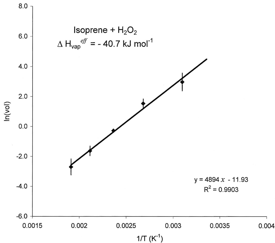
Fig. 1. Measured \Delta H_{\text{vap}}^{\text{eff}} of organic aerosol generated from the isoprene +OH reaction conducted in the absence of \text{NO}_x in Experiment 3.
