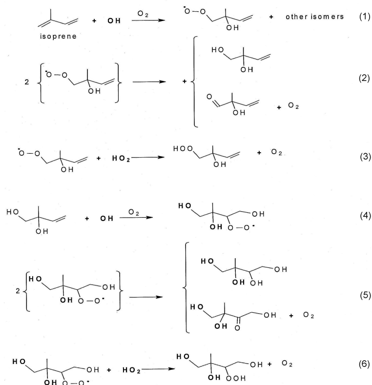
Scheme 1. Possible mechanism for the formation of methyl tetrols in the absence of NO x and acidic sulfate seed aerosol.
