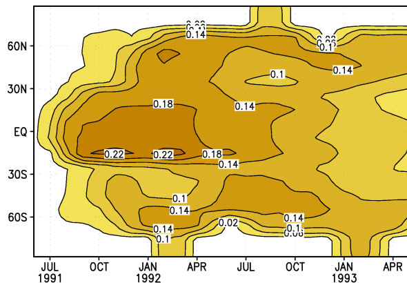
Fig. 1. Zonally averaged Pinatubo aerosol optical depth at 0.55 μm for two years after the eruption.
