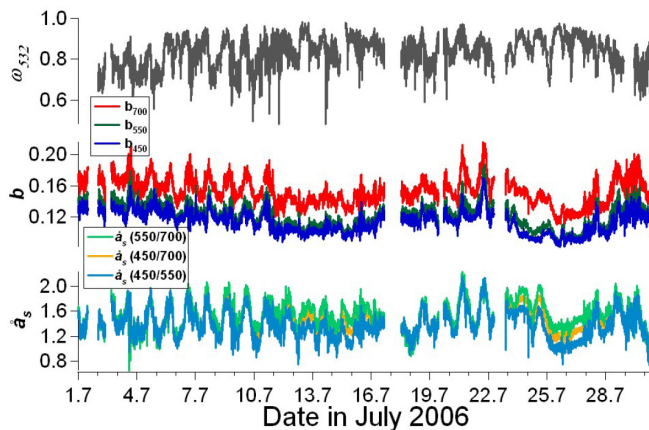
Fig. 5. Time series for the intensive optical properties: single scattering albedo ( \omega_{532} ), backscattering fraction ( b ) and Ångström exponent ( \text{Å}_s ).
