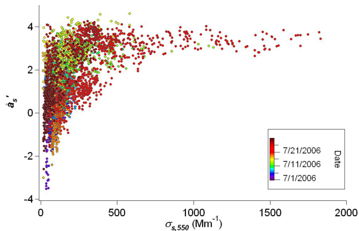
Fig. 14. Second derivative ( \dot{a}'_s ) versus scattering coefficient ( \sigma_{s,550} ) for the whole campaign, including 23–25 July.
