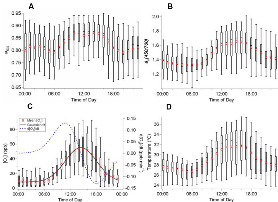
Fig. 8. Diurnal variations of (A) \omega_{532} , (B) \dot{a}_s (450/700), (C) [O_3] and d[O_3]/dt and (D) ambient temperature averaged over the campaign (excluding 23–25 July).
