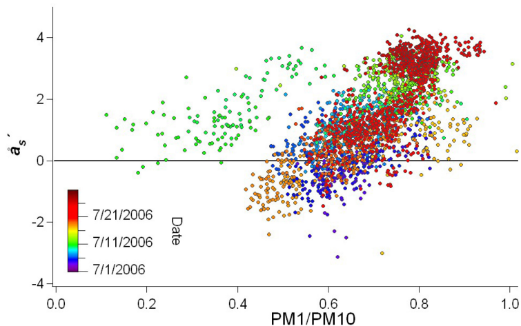
Fig. 15. Second derivative ( a'_s ) versus PM_1/PM_{10} for the whole campaign, including 23–25 July.
