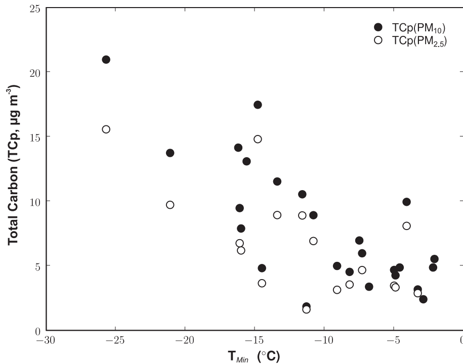
Fig. 3. Total carbon (TC p ) versus daily minimum temperature. Suburban site, Jan–Mar, 2002.
