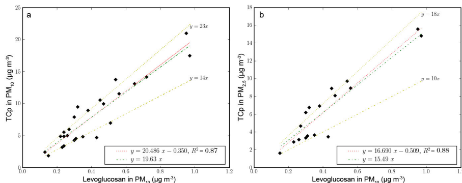
Fig. 5. Total carbon (TC p ) in PM 10 (a) and PM 2.5 (b) versus levoglucosan, as well as regression lines, a central line (no intercept) is given, and curves to capture the likely range of TC p /levoglucosan ratios indicated.
