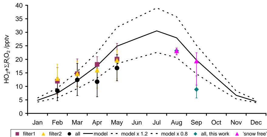
Fig. 10. Monthly median peroxy radical concentrations for all days during FREETEX, and filtered by two different methods (see Zanis et al., 2003), with data recorded during this work for all days and for “snow free” days. Error bars represent the first and third quartiles. Monthly model value on the 15th of each month is shown as a solid line, dashed lines represent model sensitivity to 20% changes in O_3 , H_2O , NO_x and photolysis rates.
