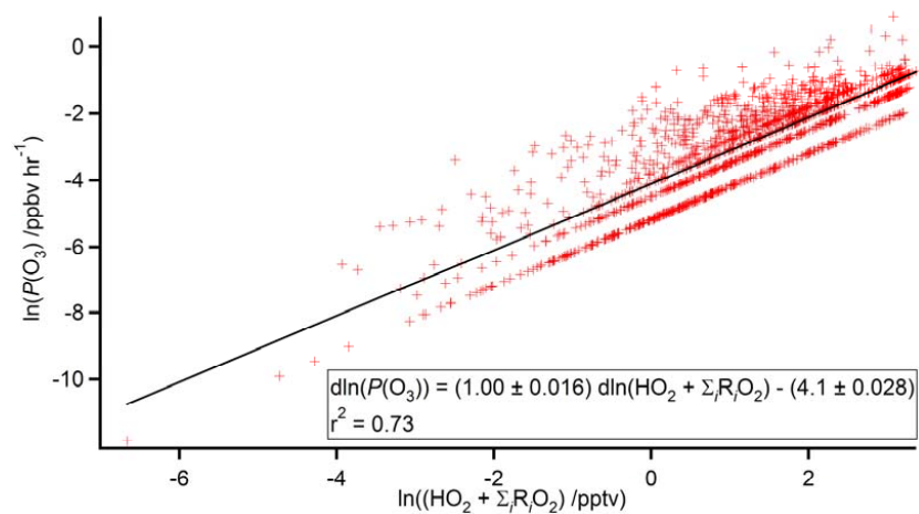
Fig. 14. Correlation between \ln(P(\text{O}_3)) and \ln(\text{peroxy radicals}) .
