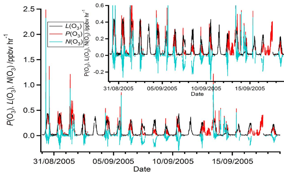
Fig. 12. Time series of P(O_3) , L(O_3) and N(O_3) .
