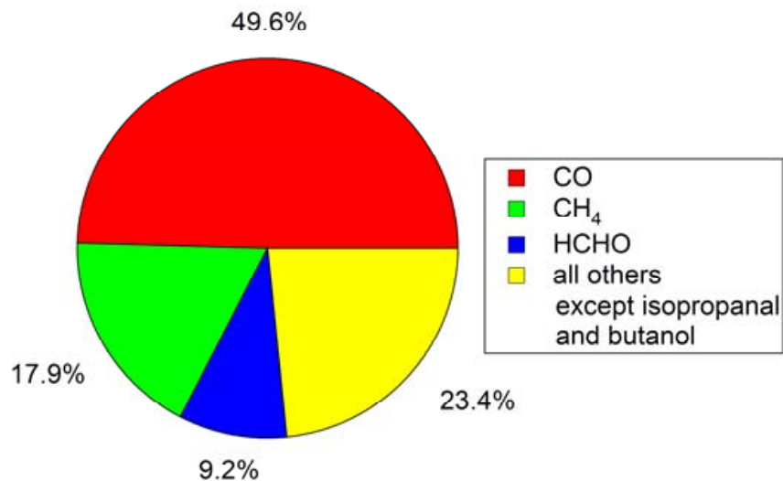
Fig. 8. Relative contributions to OH loss (with isopropanal and butanol excluded, see text).
