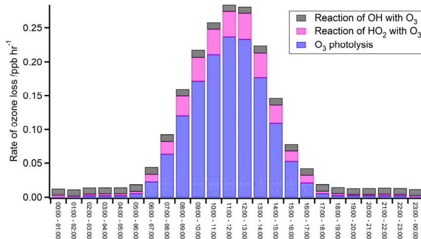
Fig. 11. Relative contributions of ozone loss terms to total L(\text{O}_3) .
