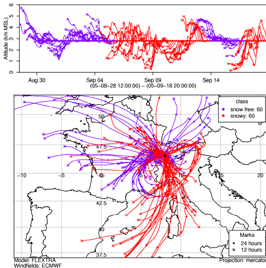
Fig. 6. Back trajectories for air masses arriving at Jungfraujoch on days classified as “snowy” and “snow free” calculated using a method adapted for use in the complex topography of the Swiss Alps (see Table 3).
