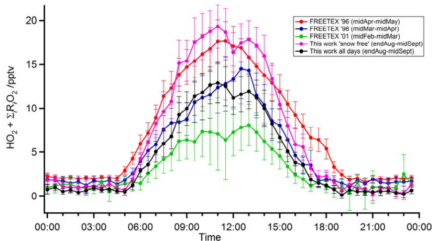
Fig. 9. Mean diurnal cycle for peroxy radicals from FREETEX'96, '98 and '01 (Zanis et al., 2003) and all days and “snow free” days from this work.
