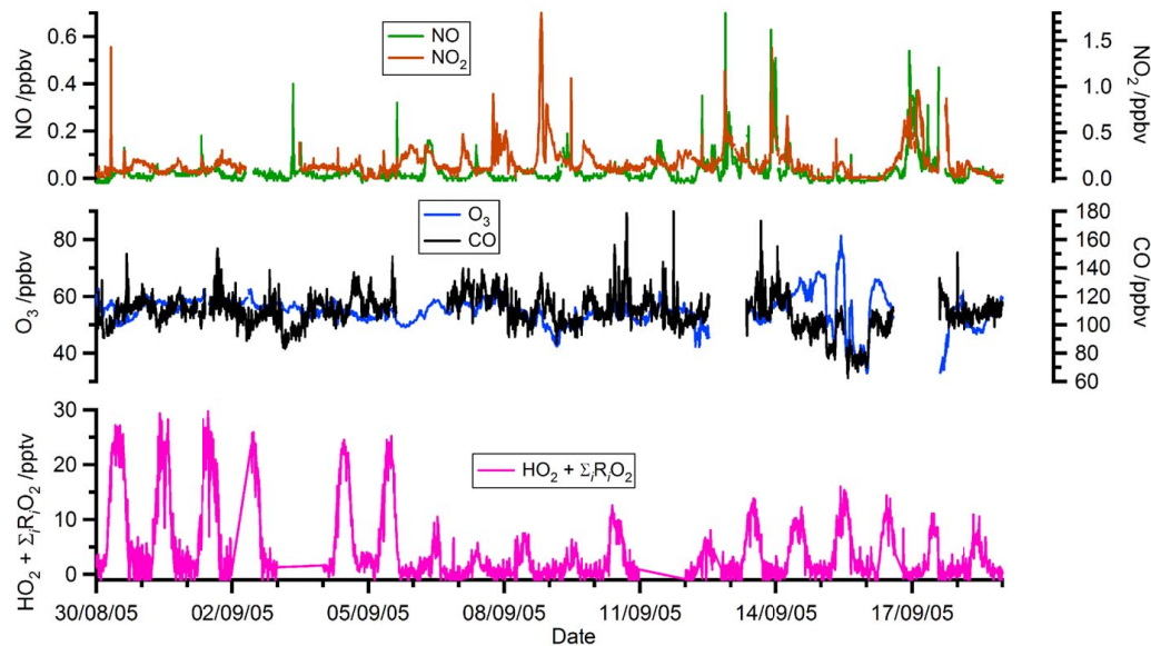
Fig. 1. Time series of peroxy radicals, O_3 , CO, NO and NO_2 measured at the Jungfraufoch from 30 August 2005–18 September 2005 inclusive.
