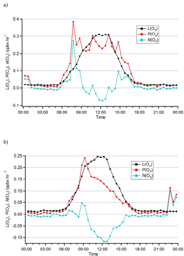
Fig. 13. (a) Mean diurnal cycle for N(O_3) , P(O_3) and L(O_3) on days classified as “snow free”; (b) mean diurnal cycle for N(O_3) , P(O_3) and L(O_3) on days classified as “snowy”.
