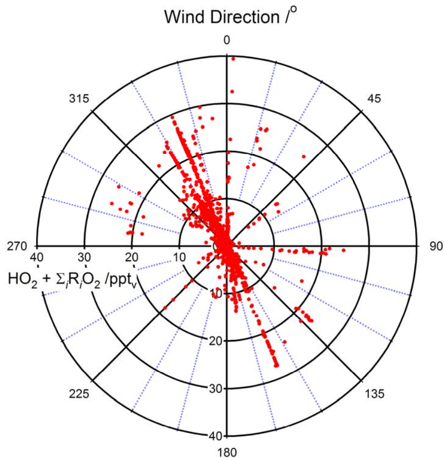
Fig. 5. Polar plot showing peroxy radical mixing ratio against wind direction.
