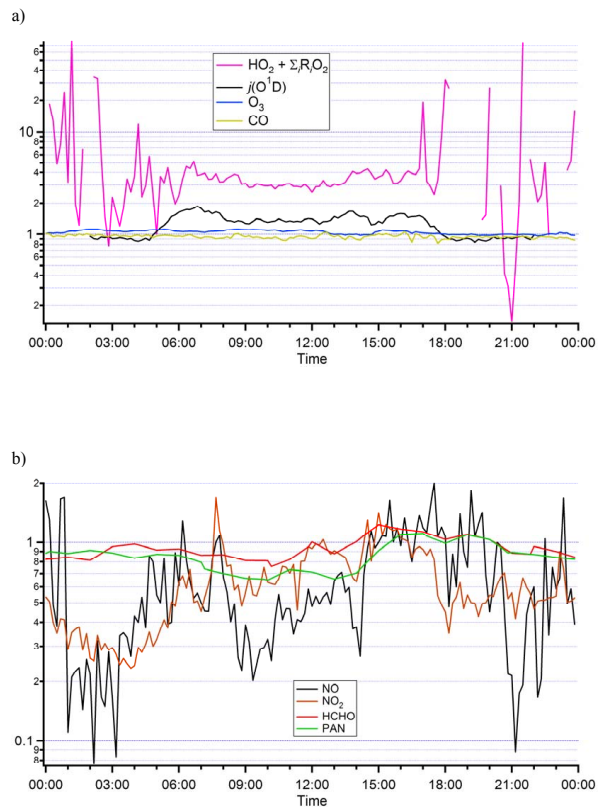
Fig. 4. (a) Mean diurnal cycle for “snow free” days divided by mean diurnal cycle for “snowy” days for peroxy radicals, j(\text{O}^1\text{D}) , ozone and CO; (b) Mean diurnal cycle for “snow free” days divided by mean diurnal cycle for “snowy” days for NO, \text{NO}_2 , HCHO and PAN.
