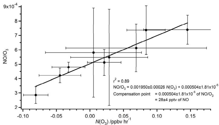
Fig. 15. Daily averaged NO/O 3 plotted against the respective daily mean N(O 3 ). The error bars represent 95% confidence limits.
