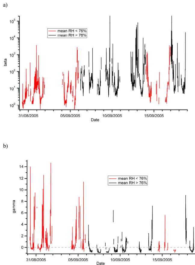
Fig. 7. (a) Time series of \beta (for definition see text); (b) time series of \gamma (for definition see text).
