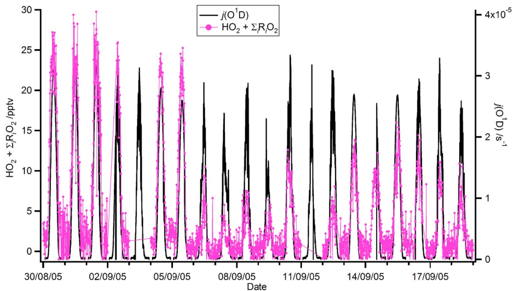
Fig. 2. Time series of peroxy radicals and j(\text{O}^1\text{D}) measurements for the period 30 August 2005 to 18 September 2005.
