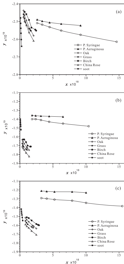
Fig. 1. Effects of various degrees of linearization. Panels (a) and (b) applies linearization from Eqs. (17a) and (19a), respectively, both without curvature adjustment; panel (c) is the same as panel (b) but with curvature adjustment. Not all species studied here are included in order to avoid cluttering of curves.
